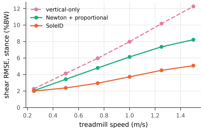
(b) Real insoles and IMUs, by treadmill speed
