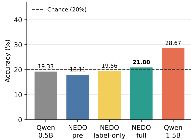
TurkishMMLU-sub
