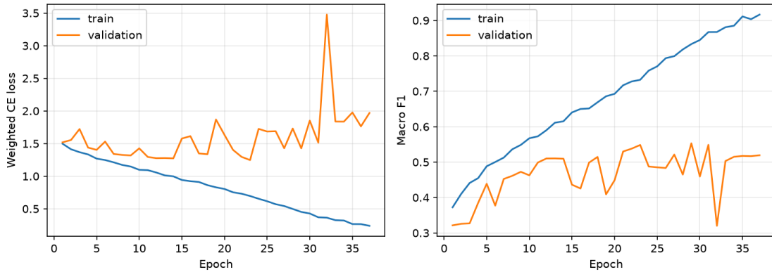
CNN winner learning curve
