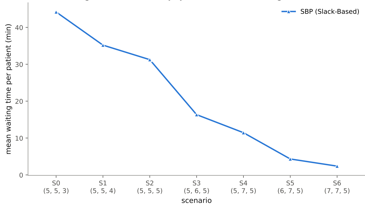
Mean waiting time across the paper's Table 10 staffing scenarios
