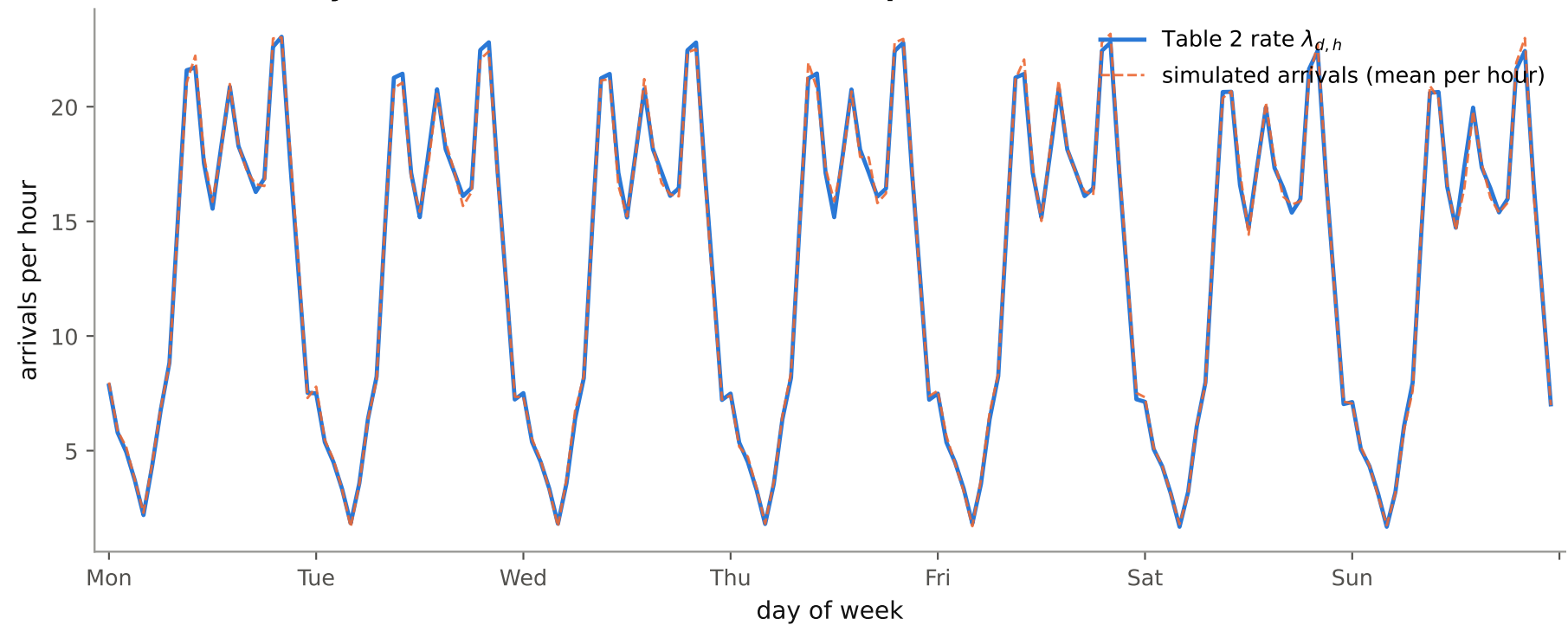
Arrival intensity: Table 2 vs the thinned NHPP sampler
