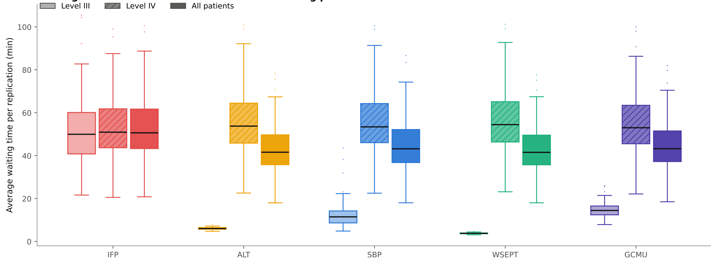
Waiting-time distributions across all five scheduling policies
