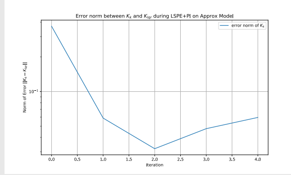
Figure 5: Convergence of K_k to K_{lqr}
