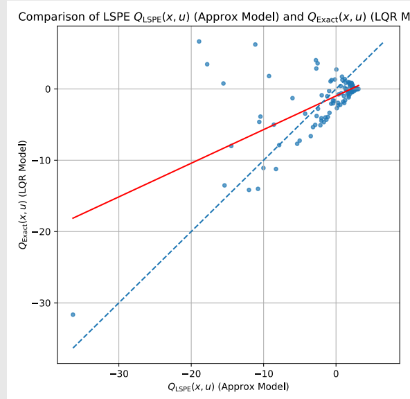
Figure 2: Exact Q -function of the LQR approximate model against Q_{\text{LSPE}}
