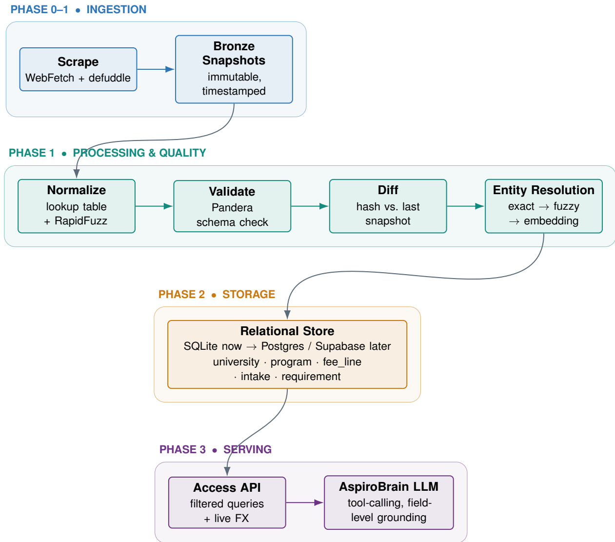
Figure 1: AspiroBrain data pipeline: four layers, each mapped to an implementation phase. Every arrow closes at least one of the seven challenges in Table 1 — normalization resolves heterogeneous formats, the diff step resolves freshness, entity resolution resolves program identity, and the storage layer’s trust-tier and verification fields feed directly into how the LLM is allowed to answer.
