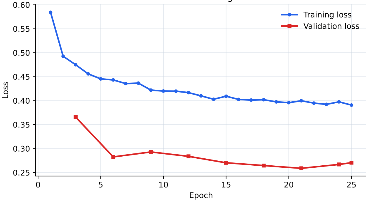
LETT-NeXt Training Loss
