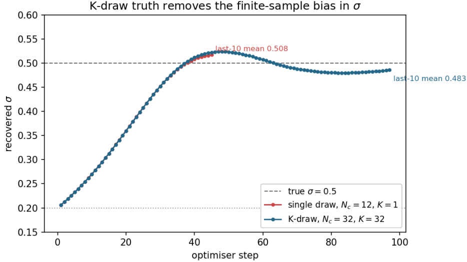
Figure 5: Recovered \sigma versus step, single-draw (red) versus K -draw (blue). Both start at 0.2 and rise together — the recovery dynamics are identical until the neighbourhood of 0.5. The single-draw curve plateaus at a last-ten mean of 0.508 ( \approx 2\% high). The K-draw curve, freed of the inflate-to-cover-an-outlier pressure, does not stop there: it overshoots slightly to \approx 0.52 (Adam momentum, not sampling) and then relaxes back , plateauing at a last-ten mean of 0.483 — last-ten and last-twenty means agree to 0.001, the signature of a genuine plateau rather than a still-drifting curve.
