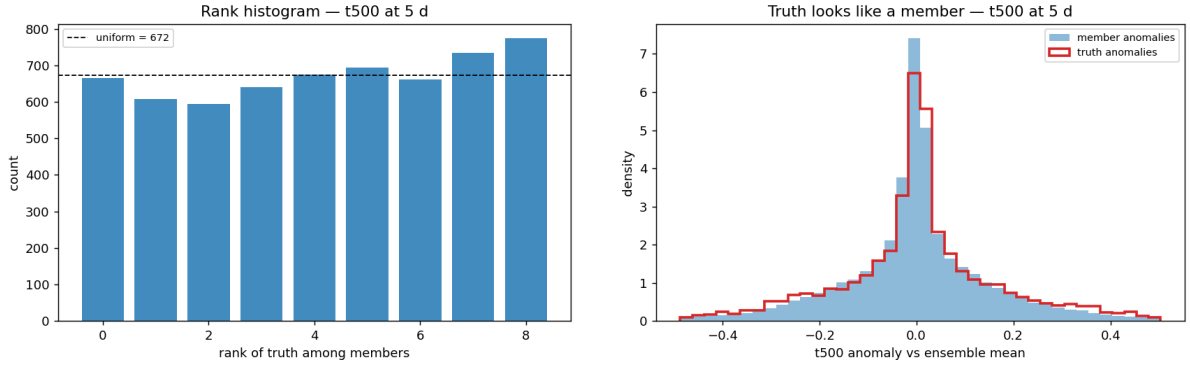
Figure 3: Left: rank histogram of t_{500} at 5 days (uniform level \approx 672 per bin). It is approximately flat with a mild upward tilt towards the higher ranks — the same slight under-dispersion (and a hint of asymmetry) seen in Table 3 — but far from the deep \cup shape of a badly under-dispersed ensemble. Right: the distribution of the members’ t_{500} anomalies (filled) with the truth’s anomalies overlaid (outline). The truth is a touch more peaked but tracks the member distribution closely: the truth looks like another draw from the ensemble.
