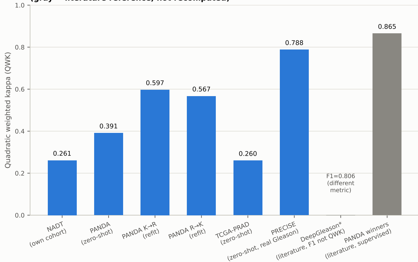
(b) QWK across cohorts vs. literature SOTA (gray = literature reference, not recomputed)
