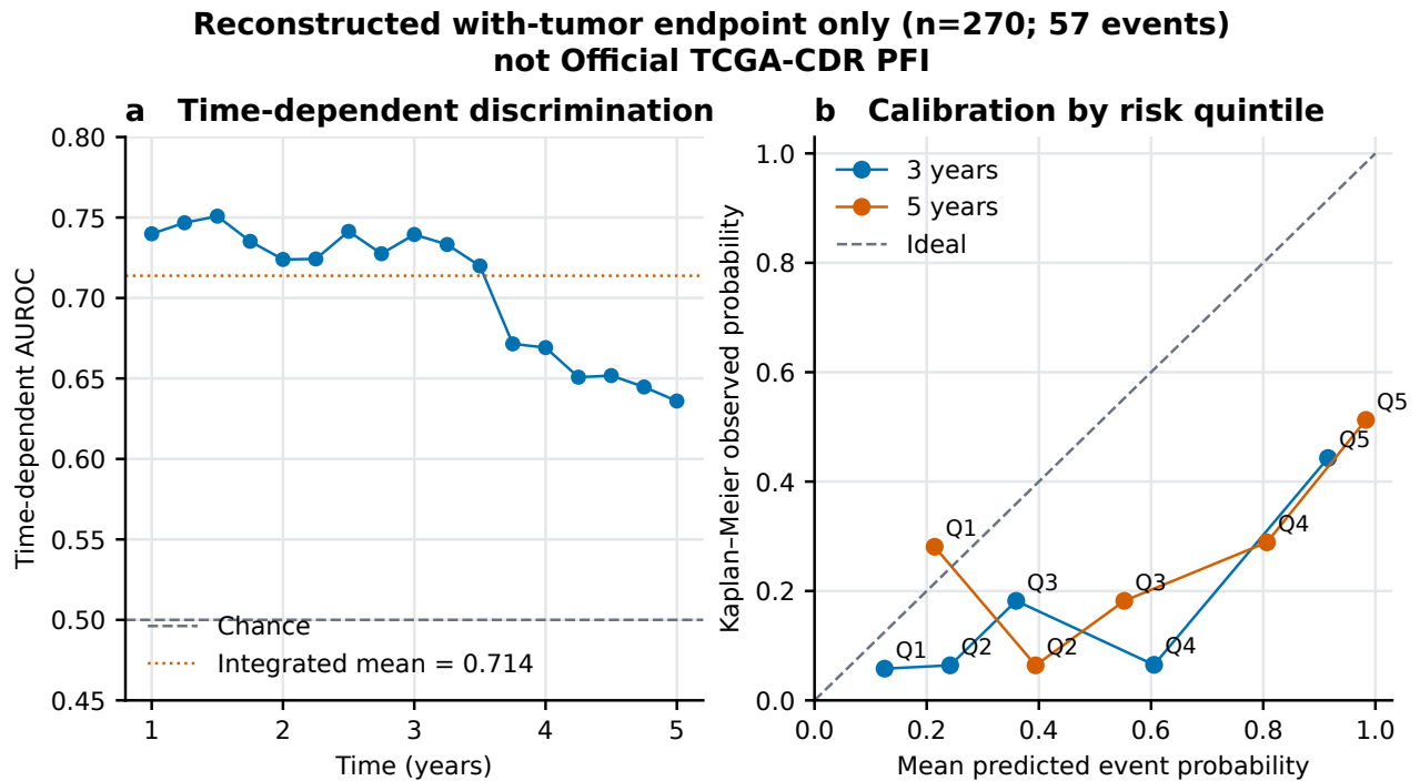
Figure S2: Legacy reconstructed-endpoint marker 7 survival summaries. Time-dependent AUROC and calibration values are rendered from the saved legacy sources for the Reconstructed with-tumor endpoint (270 patients; 57 events), not Official TCGA-CDR PFI. The endpoint name, denominator and event count were fail-closed against the saved frozen-risk metadata row and the horizon-specific calibration totals.
