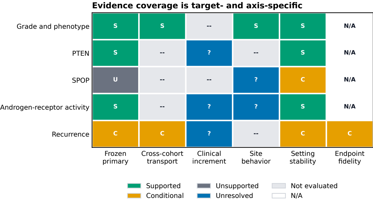
Figure S4: Target-by-axis evidence coverage. Each cell records the evidence state supported by the frozen analyses. Supported and conditional cells remain bounded to the named axis; unsupported refers to the frozen primary design, unresolved marks an evaluated question without sufficient support, and not evaluated or not applicable cells are shown explicitly rather than treated as negative evidence.
