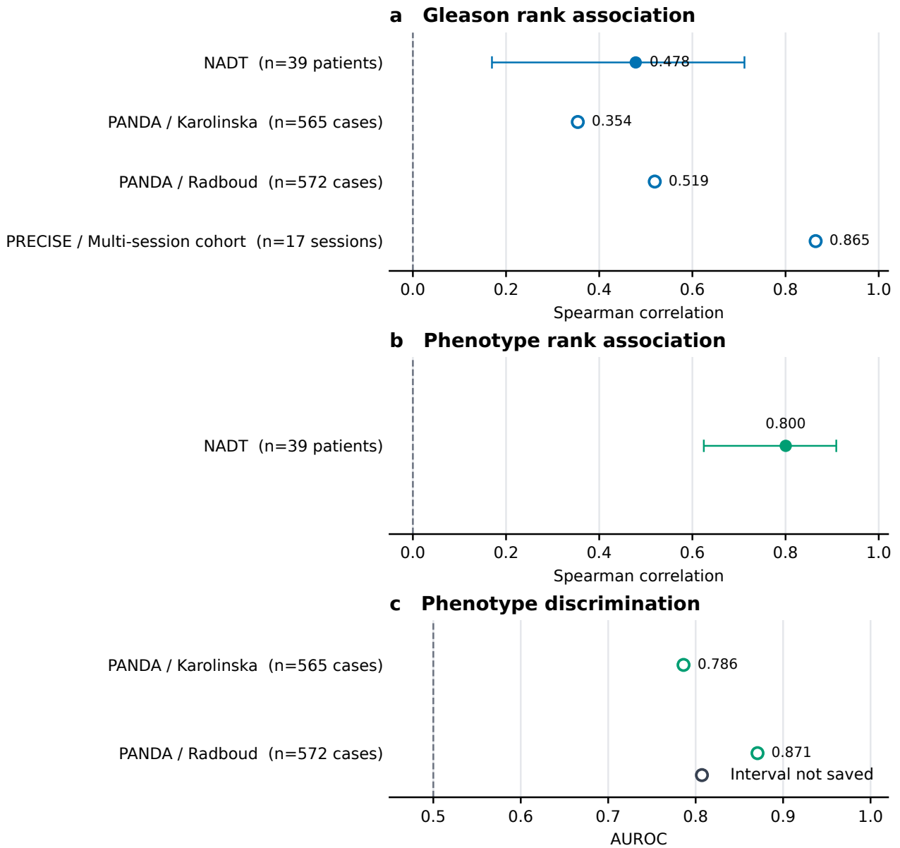
Figure S1: Saved grade and phenotype transport details. Aggregate patient-, case-image-, or session-level estimates and available uncertainty intervals are shown by target and cohort. The graphic does not imply that an unavailable interval was zero and does not convert aggregate statistics into reconstructed curves.
