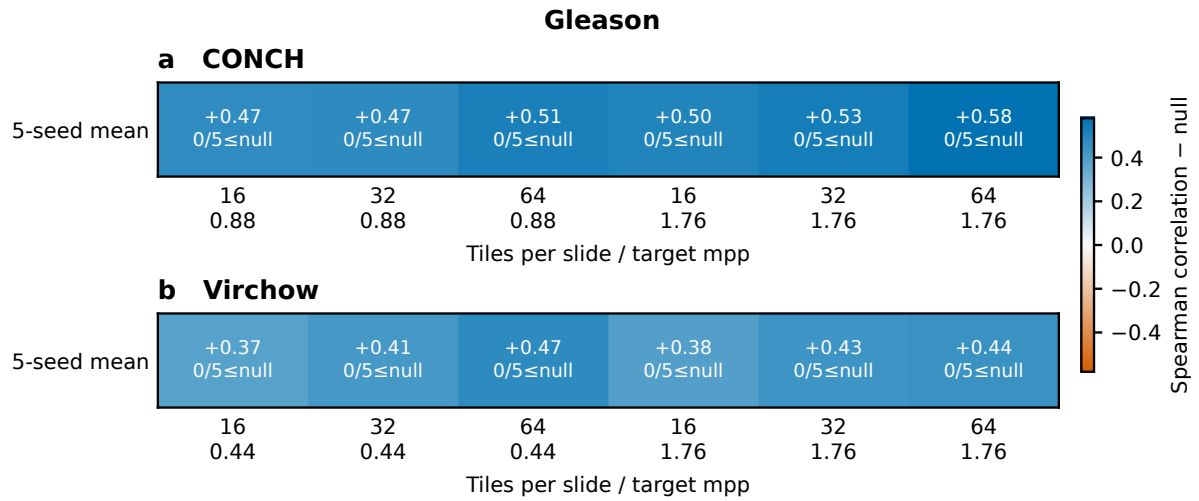
Figure S3: Complete stability grids and paired contrasts. Pages 1–6 display all 72 validated configuration means from the saved grid, one target per page. Pages 7–9 display the 390 seed-matched contrasts by comparison type. Null crossings are descriptive setting checks on reused cohorts and folds.
