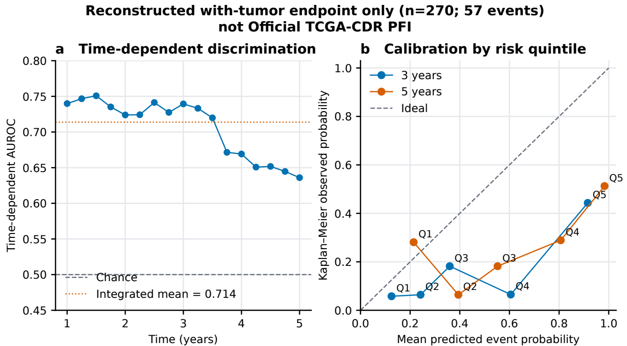
Figure S2: Legacy reconstructed-endpoint marker 7 survival summaries. Values are rendered from saved legacy sources for the Reconstructed with-tumor endpoint (270 patients; 57 events), not Official TCGA-CDR PFI. a , Time-dependent AUROC; the dashed line is chance (0.5), and the dotted line is the saved integrated mean over 1–5 years. b , Mean predicted event probability versus Kaplan–Meier observed probability by risk quintile (Q1–Q5) at 3 and 5 years; the diagonal is ideal calibration and connecting lines are visual guides across quintiles. The endpoint identity, denominator, event count, and horizon-specific calibration totals were reconciled to the saved frozen-risk metadata. This legacy summary is exploratory and supplies no Official-PFI calibration claim.
