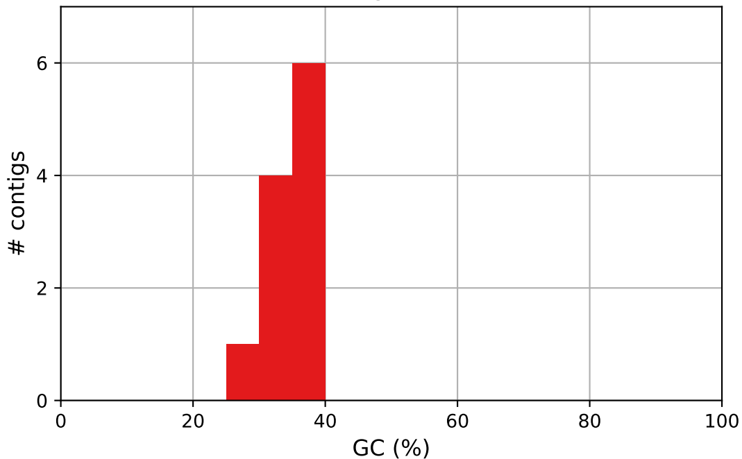
E745.contigs GC content
