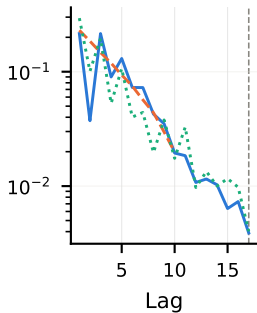
Mackey-Glass
