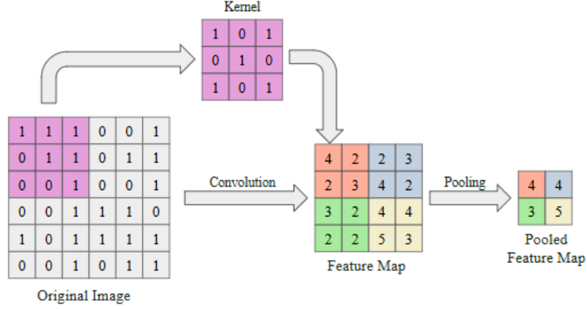
Figure 15: Example of convolutional neural network operations. convolutional kernel slides across the input image and performs a dot product with local pixel values to produce a feature map highlighting the presence of specific patterns. In typical CNN architectures, a nonlinear activation function such as ReLU is applied after convolution. A pooling layer may then downsample the feature map while preserving the strongest activations. Figure adapted from [57].
