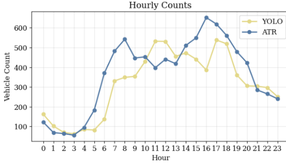
(c) Atlantic Avenue at Boerum Place. Raw hourly counts.
