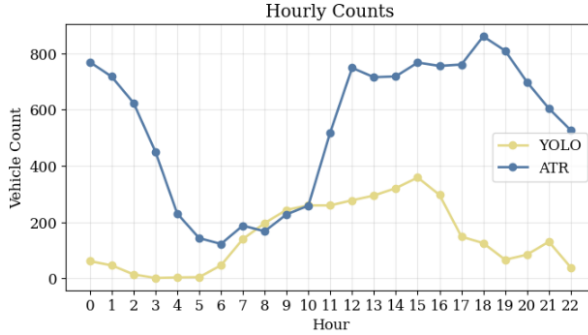
(e) Broadway at Houston. Raw hourly counts.
