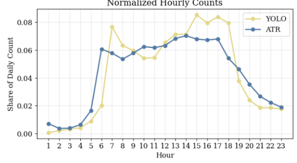
(b) Pelham Parkway Westbound at Boston Road. Normalized hourly counts.
