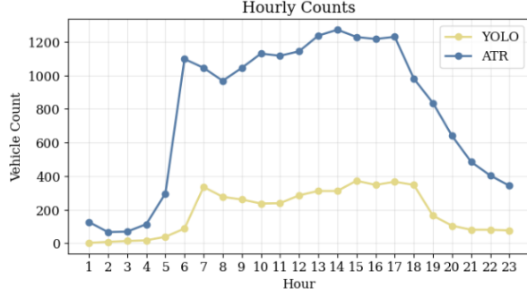
(a) Pelham Parkway Westbound at Boston Road. Raw hourly counts.
