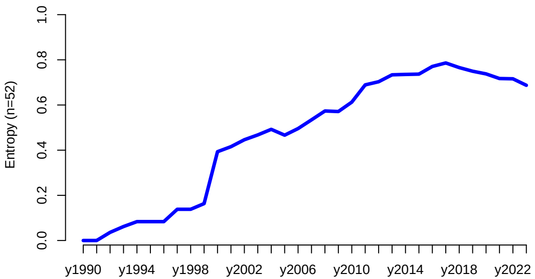
Transport – state entropy
