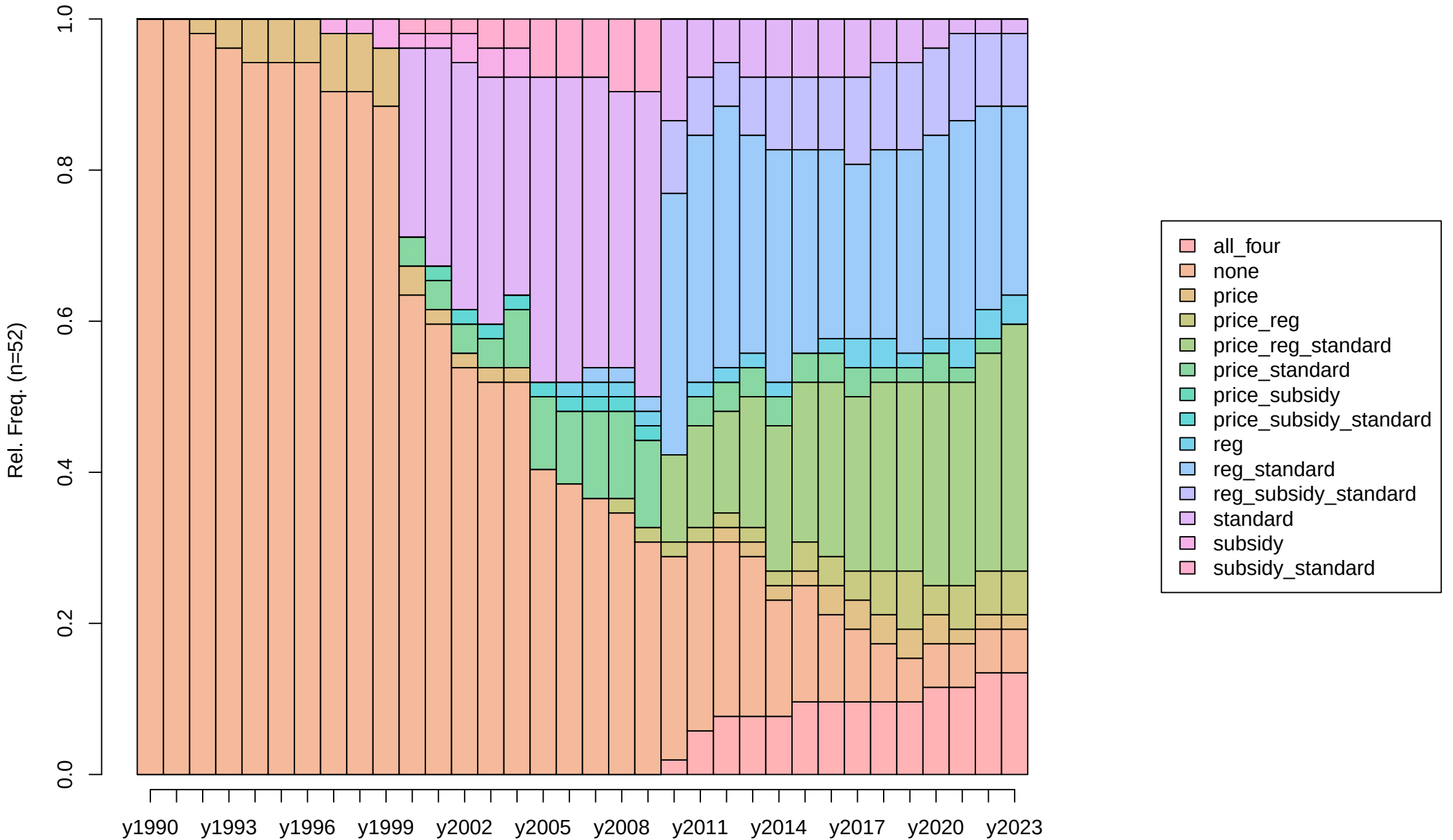
Transport – state distribution
