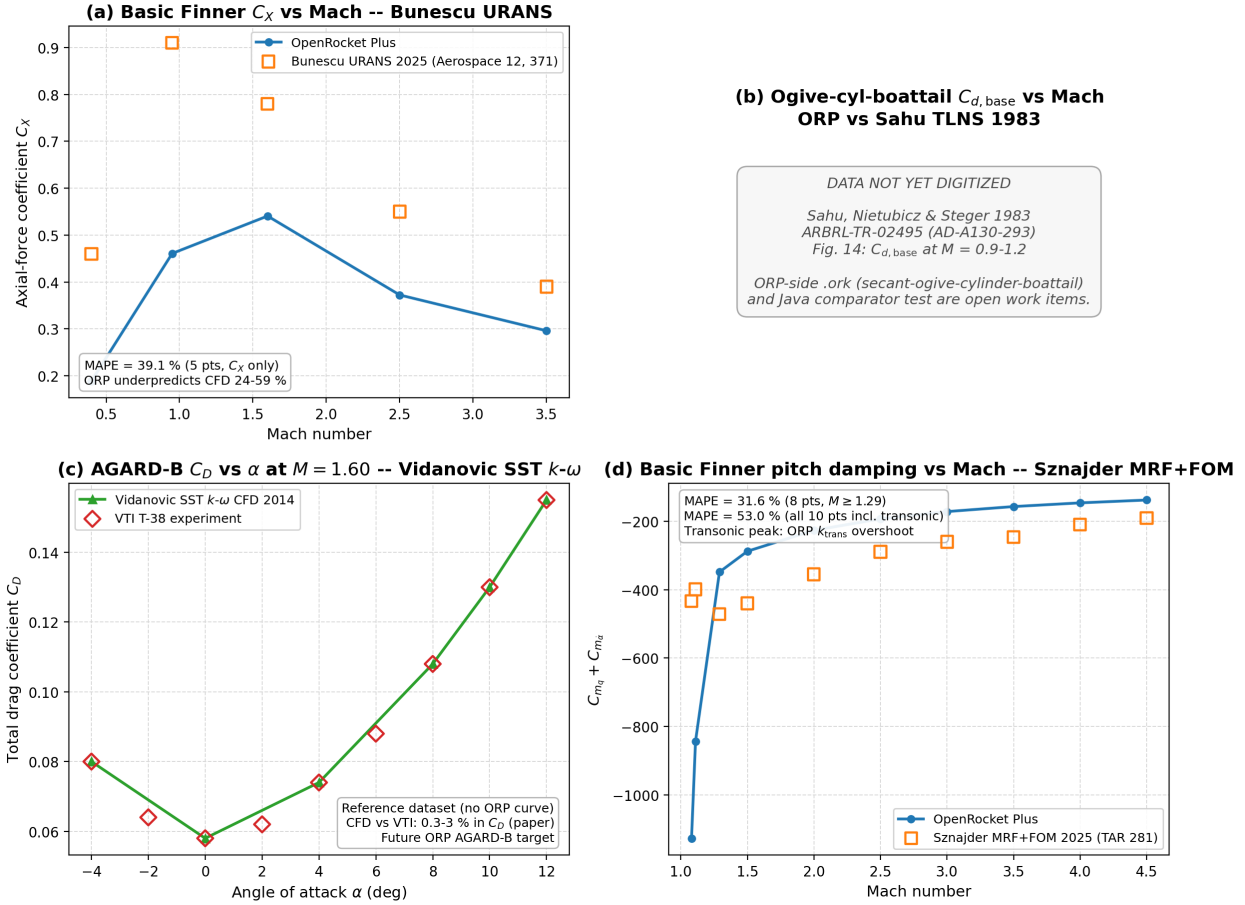
Fig. 19 Published-CFD comparator composite. Panel A: Basic Finner axial-force coefficient versus the Bunescu URANS solution [43] (correct trend, loose absolute agreement). Panel B: ogive-cylinder-boattail base drag versus the Sahu thin-layer Navier–Stokes solution [44] (digitization deferred). Panel C: AGARD Model B reference dataset versus the Vidanović SST k-\omega solution and VTI T-38 experiment [45]. Panel D: Basic Finner pitch-damping sum versus the Sznajder Fluent solution [37], cross-corroborated on the AFF and ANF finner planforms by the CFD++ study of Bhagwandin and Sahu [42].
