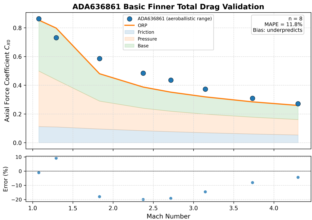
Fig. 18 Finned-vehicle total drag for the Army–Navy Basic Finner reference projectile versus the Dupuis and Hathaway ballistic-range data [40], M = 1.08 –4.30. Aggregate MAPE 11.8% over eight points.
