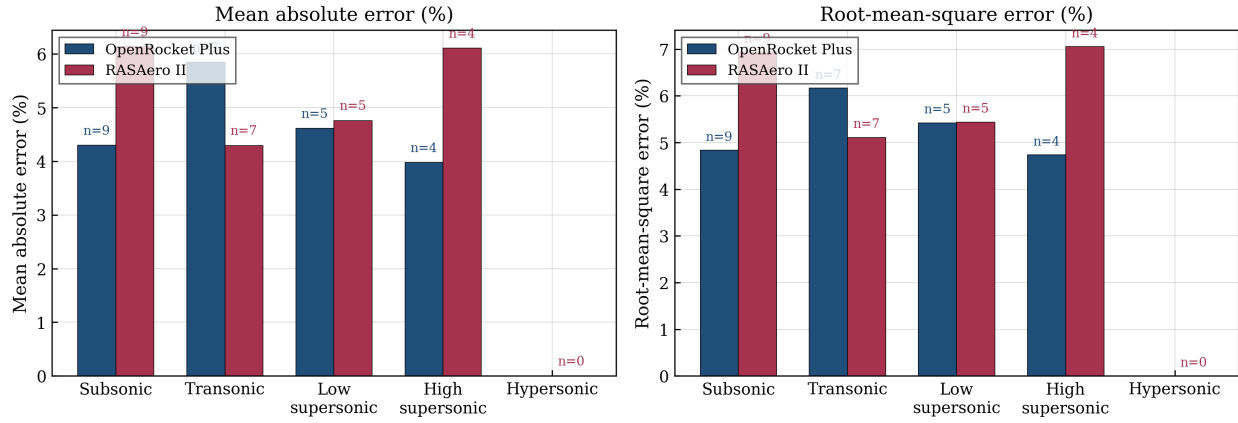
Fig. 23 Per-regime error distribution. The transonic band carries the largest negative bias; the high-supersonic band has the tightest scatter. Bands above Mach 3 contain four or fewer flights and are descriptive only.
