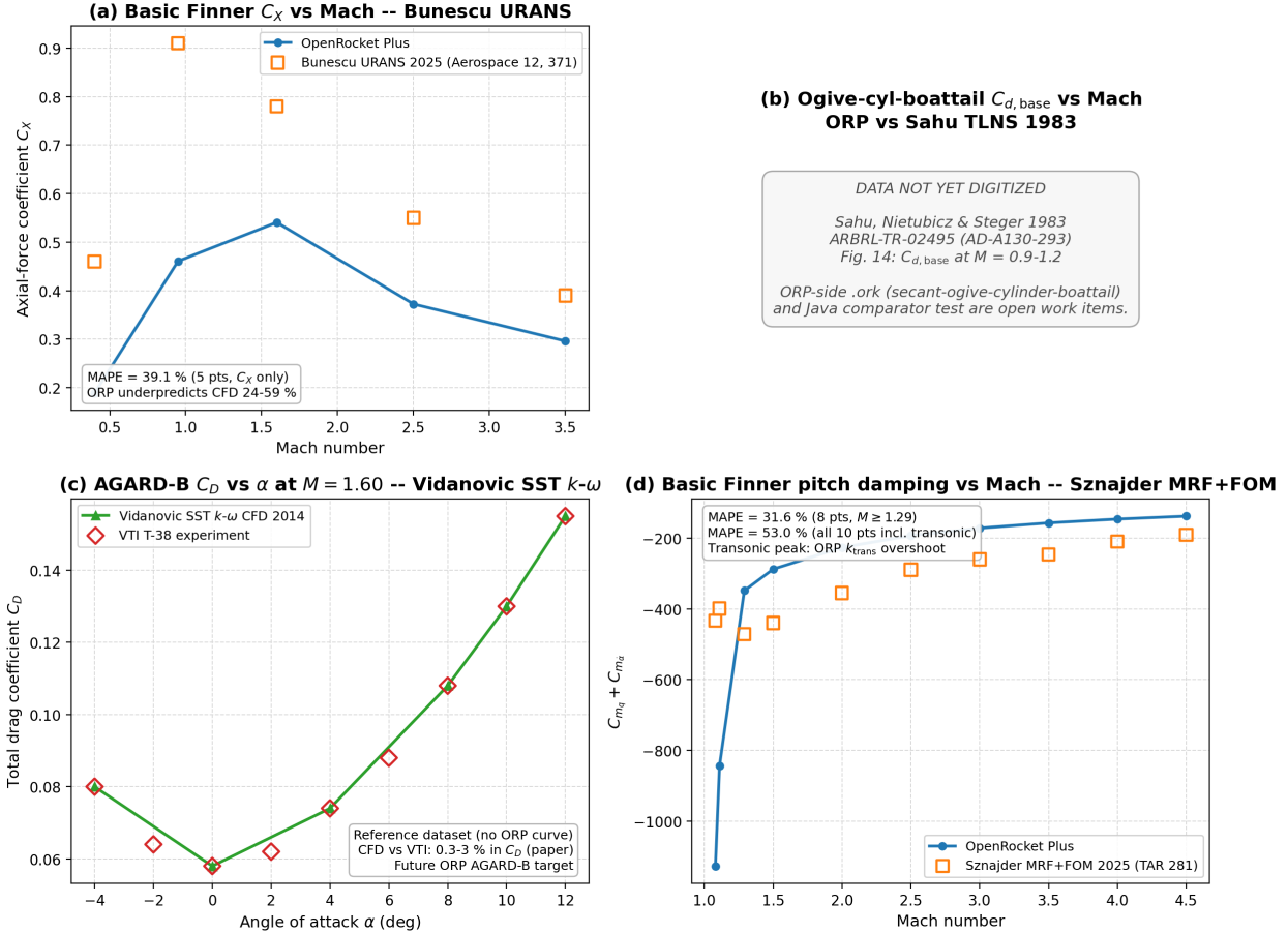
Fig. 20 Published-CFD comparator composite. Panel A: Basic Finner axial-force coefficient versus the Bunescu URANS solution [40] (correct trend, loose absolute agreement). Panel B: ogive-cylinder-boattail base drag versus the Sahu thin-layer Navier–Stokes solution [41] (digitization deferred). Panel C: AGARD Model B reference dataset versus the Vidanović SST k-\omega solution and VTI T-38 experiment [42]. Panel D: Basic Finner pitch-damping sum versus the Sznajder Fluent solution [35], corroborated by Bhagwandin and Sahu [43].
