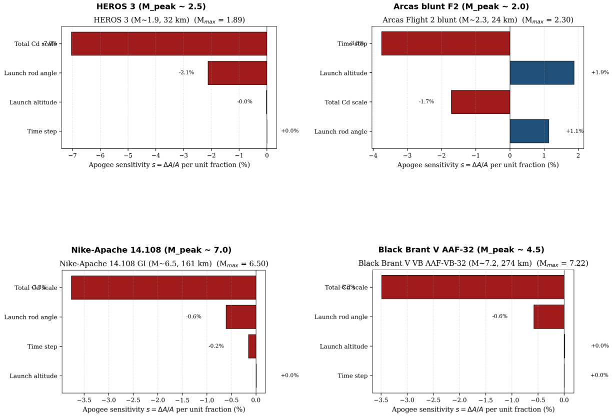
Fig. 27 Sensitivity tornado composite for the four high-Mach exploratory vehicles (HEROS 3, blunt Arcas, Nike-Apache, Black Brant VB) under \pm 10\% perturbations of drag-coefficient scale, integration time step, launch altitude, and launch-rod angle. These worst-case trajectories bound the numerical-convergence behavior of the gentler headline flights; drag-coefficient scale dominates the response.
