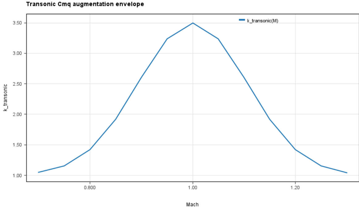
Fig. 17 Transonic Gaussian augmentation k_{\text{transonic}}(M) of the pitch-damping derivative, Eq. (29), peaking at 3.5\times at M = 1 and decaying to unity within \pm 0.3 Mach. The augmentation is a B-level adjustment with no independent wind-tunnel anchor; the size of the closure correction overshoots the physical transonic damping peak by an estimated 110–160% [35].
