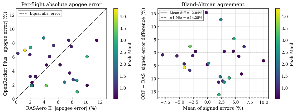
Fig. 26 Paired per-flight comparison of OpenRocket-Plus and RASAero II apogee errors. The paired absolute-error difference is statistically indistinguishable from zero (Wilcoxon p = 0.615 ), supporting a parity conclusion.
