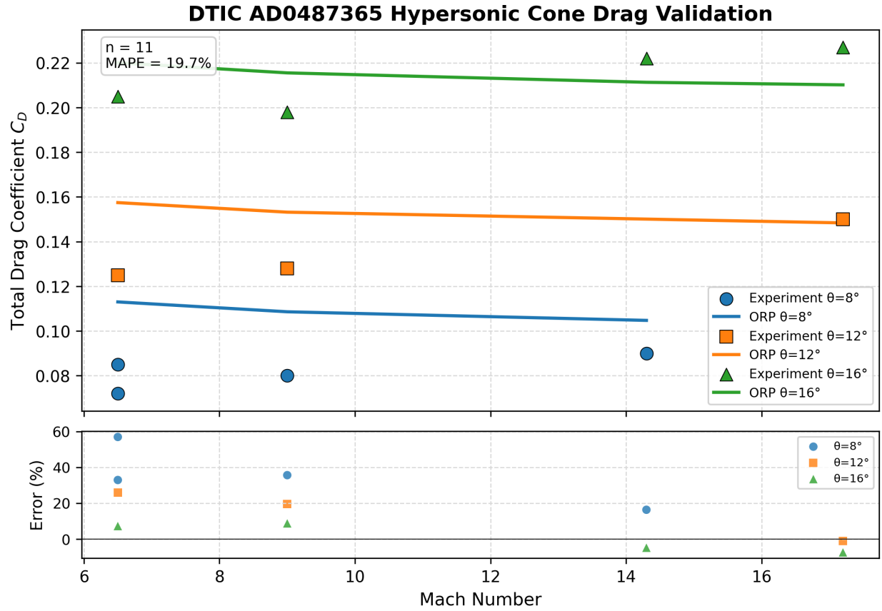
Fig. 14 Hypersonic cone foredrag versus DTIC AD0487365 [29] ballistic-range data, M = 6.5\text{--}17.2 , half-angles 8, 12, and 16 deg. Aggregate mean absolute percentage error = 19.7% over 11 points; the largest residual is +57% for the thinnest cones at the lowest Reynolds number.
