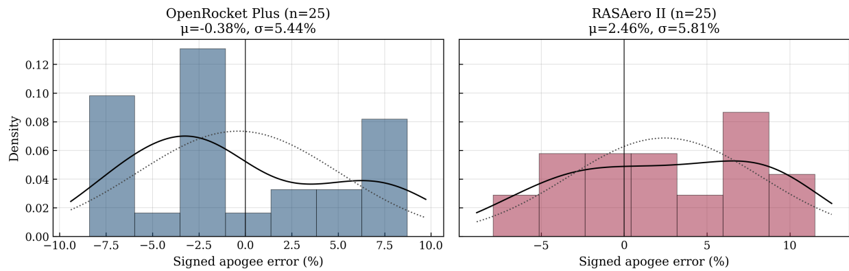
Fig. 24 Error distributions for OpenRocket-Plus and RASAero II on the 25-flight corpus. Both are light-tailed; the ORP distribution centers near zero.
