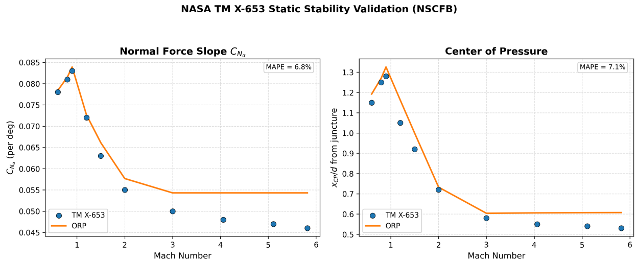
Fig. 15 Static stability against the NASA TM X-653 wind-tunnel database [32], M = 0.6\text{--}5.82 : finned-body normal-force slope C_{N_\alpha} and center-of-pressure location x_{CP}/d . The local-flow model achieves C_{N_\alpha} MAPE 6.84% and x_{CP}/d MAPE 7.11% over ten test points each, with the largest residual confined to the transonic band.
