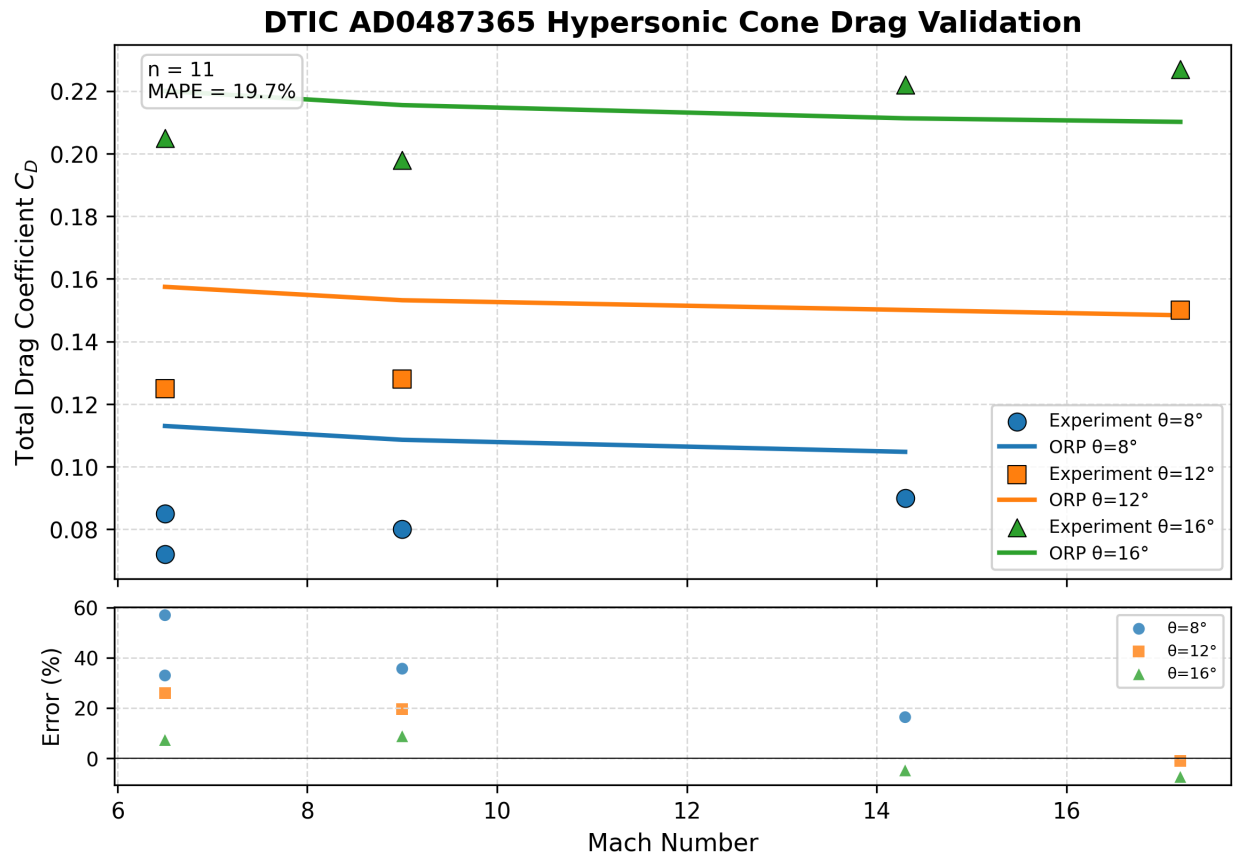
Fig. 19 Hypersonic cone-cylinder foredrag versus the DTIC AD0487365 range tests [29], M = 6.5\text{--}17.2 , source Reynolds number matched row by row. Aggregate MAPE 19.7%; the largest single residual (+57%) occurs on the thinnest, lowest-Reynolds-number cone. Reported as an exploratory hypersonic extension of a supersonic-validated method.
