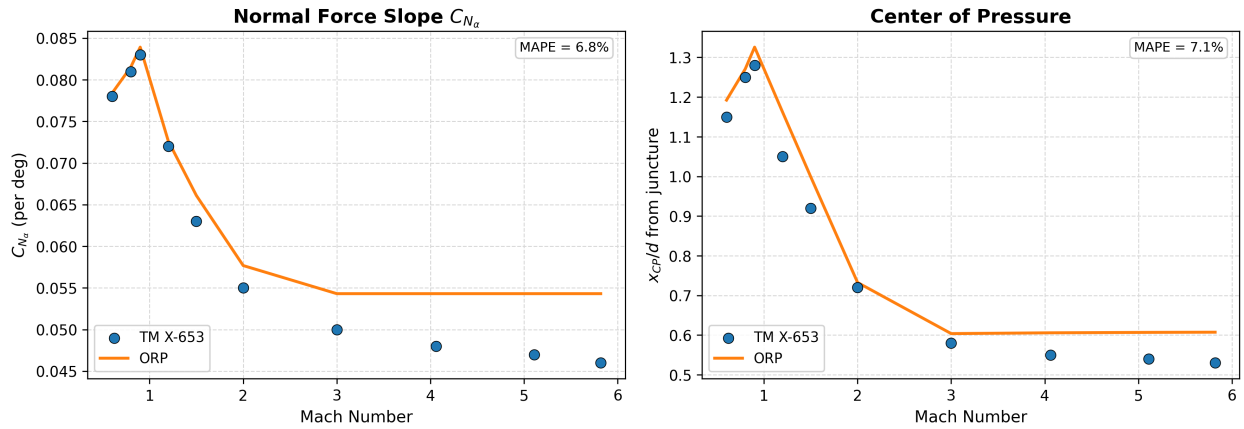
Fig. 15 Static stability against the NASA TM X-653 wind-tunnel database [33], M = 0.6\text{--}5.82 : finned-body normal-force slope C_{N_\alpha} and center-of-pressure location x_{CP}/d . The local-flow model achieves C_{N_\alpha} MAPE 6.84% and x_{CP}/d MAPE 7.11% over ten test points each, with the largest residual confined to the transonic band.
