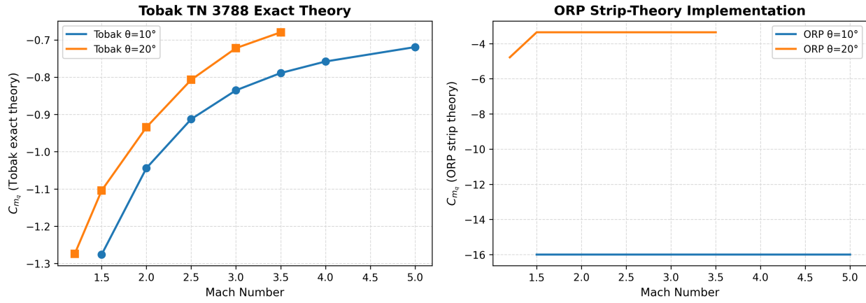
Fig. 16 Strip-theory pitch-damping derivative C_{mq} compared with the exact slender-body theory of Tobak and Wehrend, NACA TN 3788 [35]. The sign is correct and the damping is conservative, but strip theory overpredicts the magnitude for an isolated axisymmetric body by a factor of five to ten; the derivative is therefore reported as a conservative engineering estimate rather than a quantitative result.
