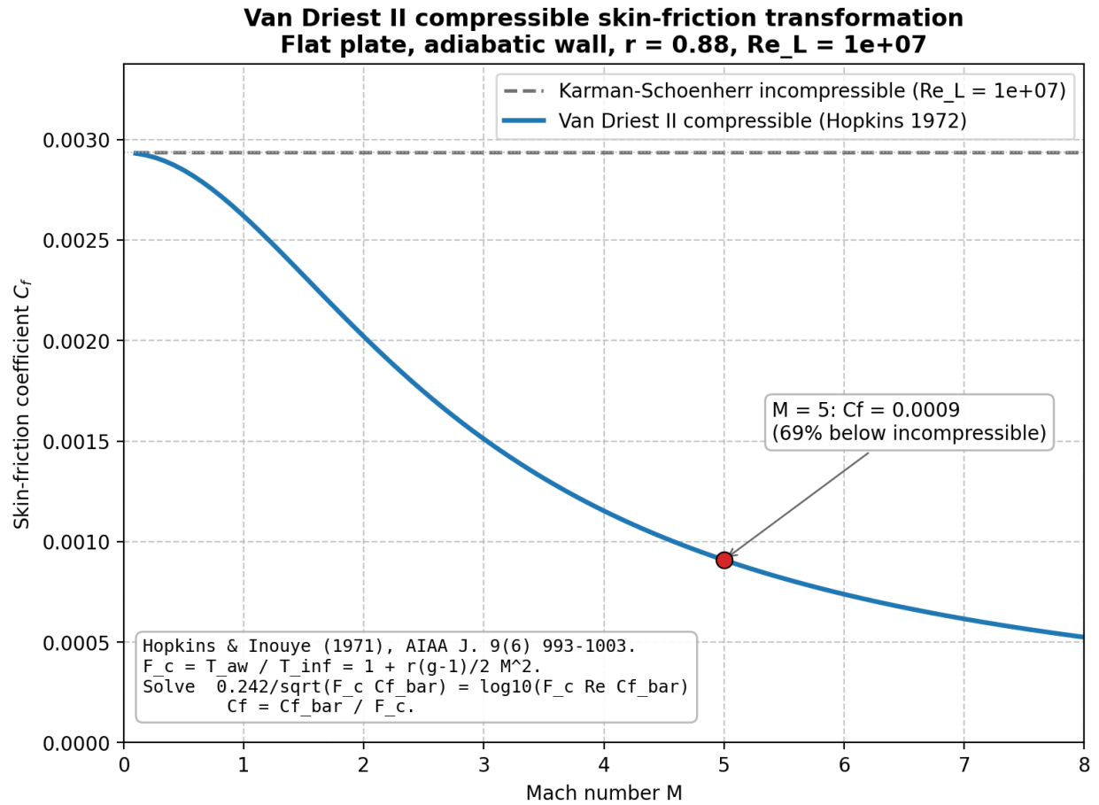
Fig. 13 Van Driest II compressible skin-friction coefficient versus Mach number for a representative slender body at length Reynolds number Re_L = 10^7 , after the Hopkins–Inouye formulation [17].
