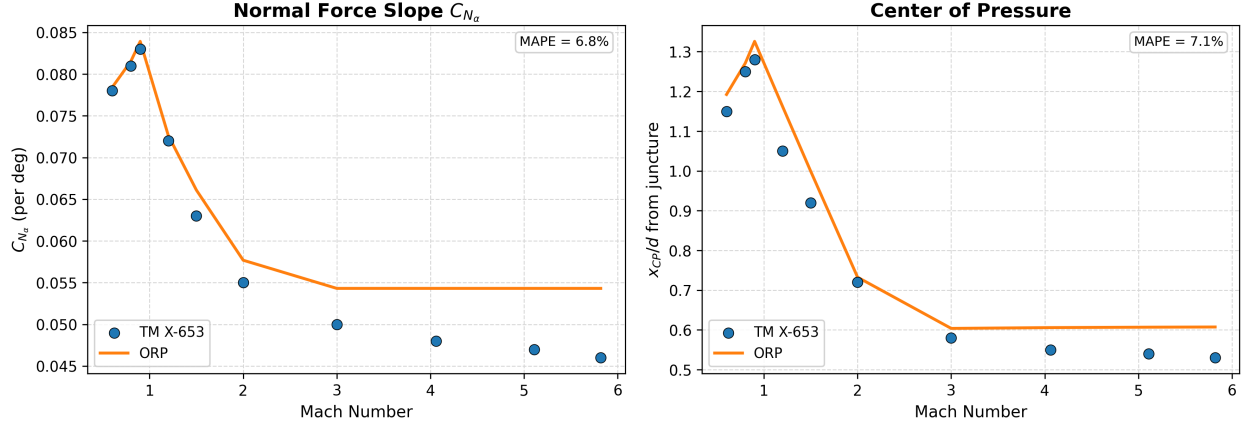
Fig. 15 Static stability against the NASA TM X-653 wind-tunnel database [34], M = 0.6 – 5.82 : finned-body normal-force slope C_{N_\alpha} and center-of-pressure location x_{CP}/d . The local-flow model achieves C_{N_\alpha} MAPE 6.84% and x_{CP}/d MAPE 7.11% over ten test points each, with the largest residual confined to the transonic band.
