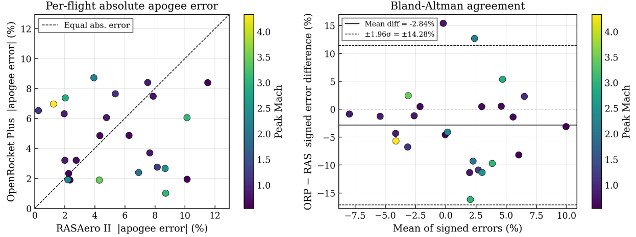
Fig. 25 Paired per-flight comparison of OpenRocket-Plus and RASAero II apogee errors. The paired absolute-error difference is statistically indistinguishable from zero (Wilcoxon p = 0.615 ), supporting a parity conclusion.
