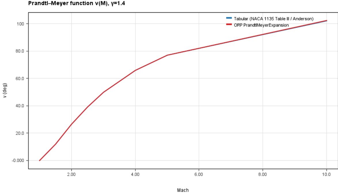
Fig. 8 Prandtl-Meyer function v(M) , Eq. (11), versus NACA Report 1135 Table III.
