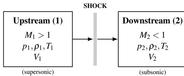
Figure 3: Stationary normal shock: control volume spanning the thin shock region.
