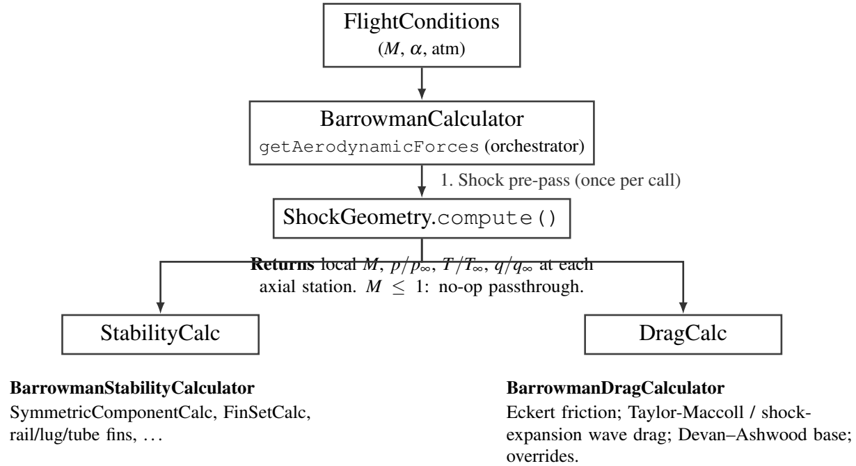
Figure 1: Aerodynamic evaluation pipeline: ShockGeometry is computed once per call and shared with stability and drag sub-calculators.
