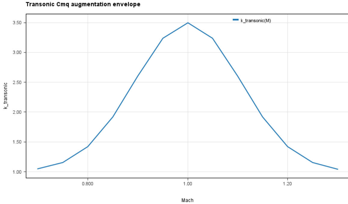
Fig. 17 Transonic Gaussian augmentation k_{\text{transonic}}(M) of the pitch-damping derivative, Eq. (27), with peak augmentation parameter k(1.0) = 3.5 at M = 1 and decaying to unity within \pm 0.3 Mach. The accompanying 3 \times C_{mq} multiplier is a B-level adjustment calibrated against the AEDC-TR-76-58 transonic pitch-damping wind-tunnel data with no independent flight-scale anchor; at M = 1.08 – 1.11 the augmented model overshoots the physical transonic damping peak resolved by the Sznajder CFD by an estimated 110–160% [37].
