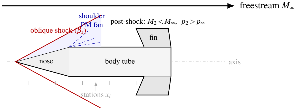
Figure 12: Shock and expansion topology on a cone-cylinder-fin vehicle (schematic).
