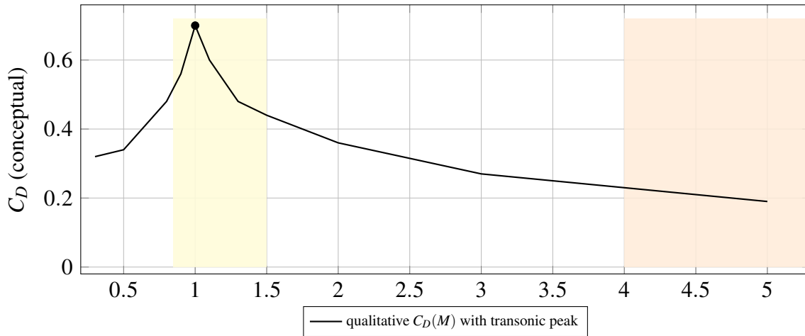
Figure 18: Conceptual total drag coefficient vs Mach (not a specific vehicle). Shaded band M \in [0.85, 1.50] highlights the dense transonic overlap of blend regions; M \in [4, 6] indicates the Modified Newtonian transition (Section 10.4 catalog).
