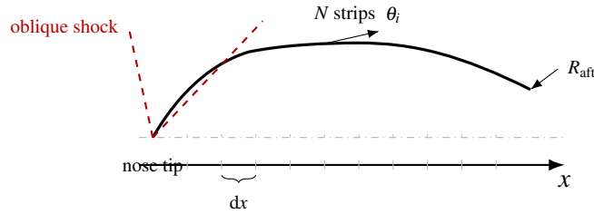
Figure 8: Shock-expansion strip model along an ogive (schematic).
