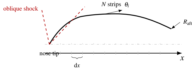
Figure 8: Shock-expansion strip model along an ogive (schematic).
