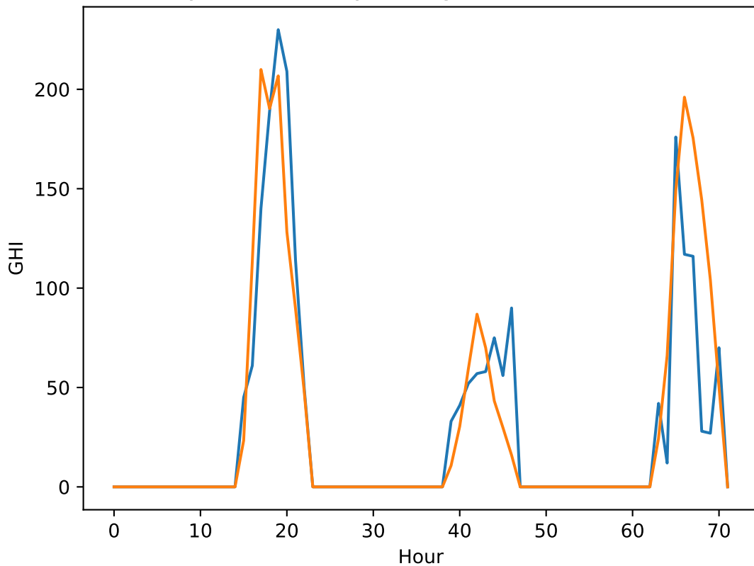
Day of Year Hourly Average GHI Pred vs Actual
