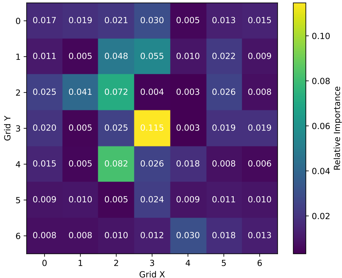
XGBoost Feature Importance by Point
