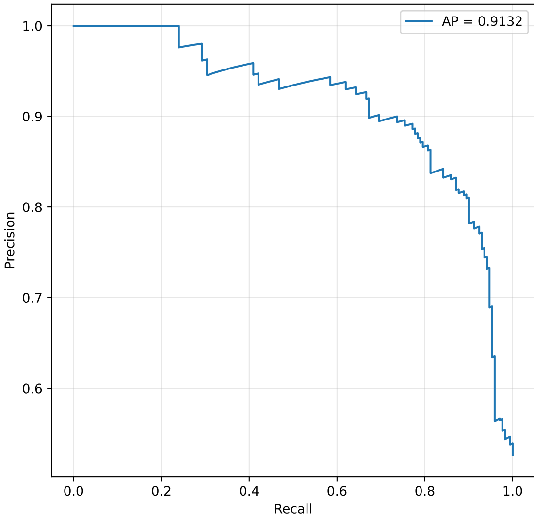
Precision-Recall Curve
