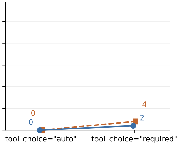
Tasks resolved
