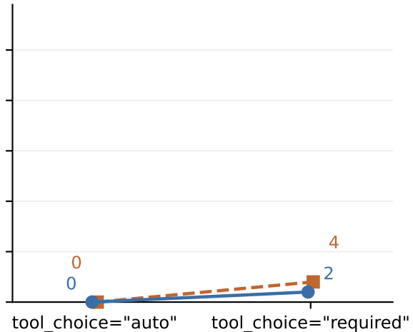
Tasks resolved
