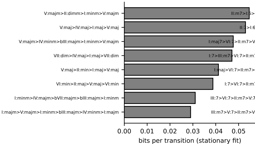
Bach chorales: fundamental-cycle terms j_{CA_C} (top-5 share 18.2%)
