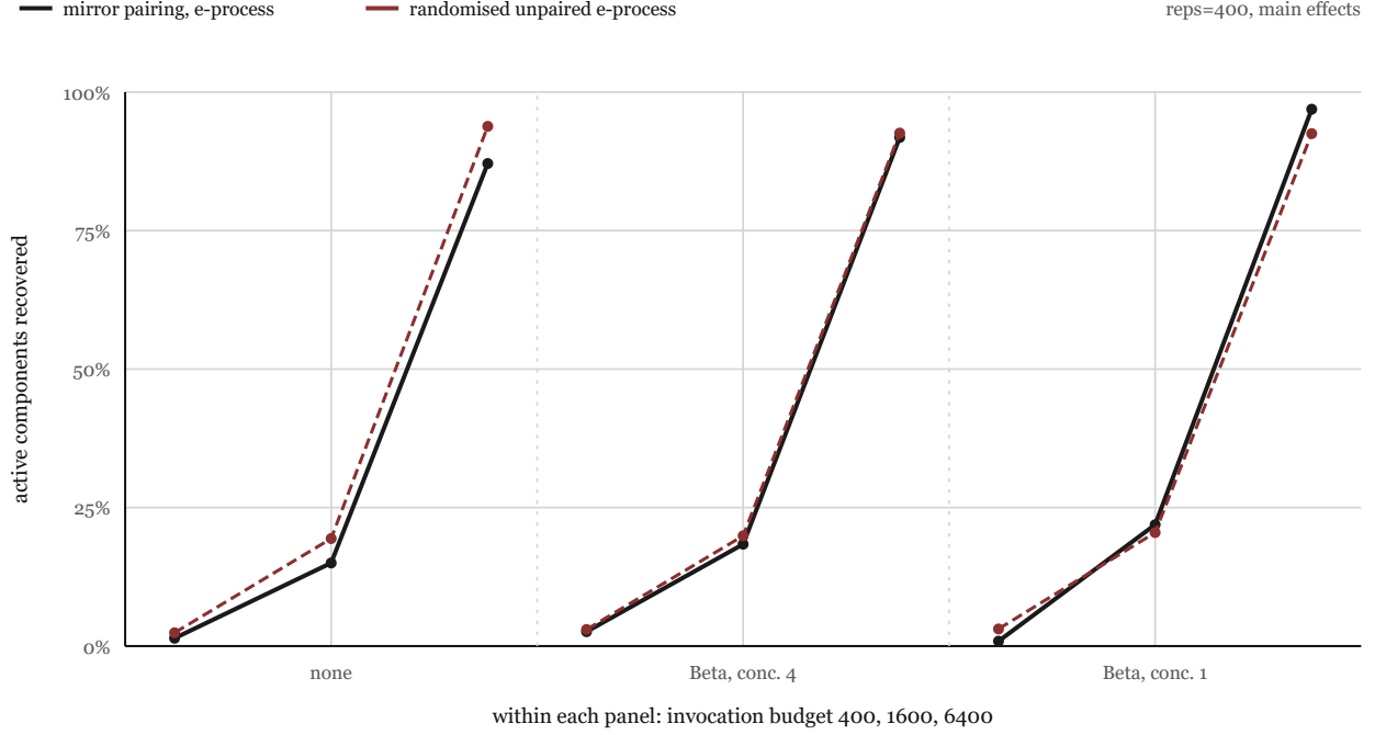
Figure 8. Recovery of the two active components by task-difficulty spread, k = 5 , main effects. With homogeneous tasks the unpaired procedure matches the mirror at half the invocations per row; as the spread grows the task effect stays inside every unpaired increment and the mirror pulls away.
