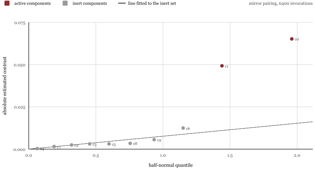
Figure 7. The standard screening plot for one run at ten components: absolute estimated contrasts against half-normal quantiles. The eight inert components lie on a line through the origin, the two active ones leave it. This is the diagnostic a practitioner reads before deciding what to keep.
