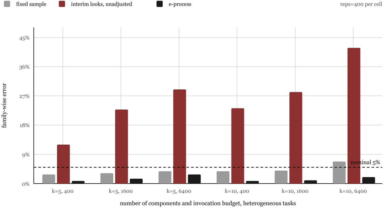
Figure 3. False admission of an inert component under the global null, by budget and number of components. Unadjusted interim analysis is far above the nominal level everywhere; the e-process is below it everywhere.
