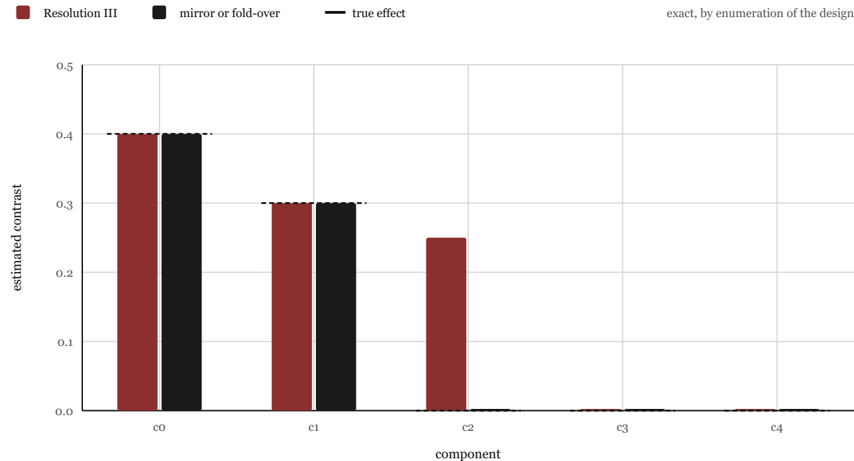
Figure 2. Contrast recovered per component with one two-factor interaction of 0.25 between components 0 and 1, computed exactly by enumerating each design. The Resolution III design credits the whole interaction to inert component 2; the mirror difference and the fold-over design return the true effect on every component.
