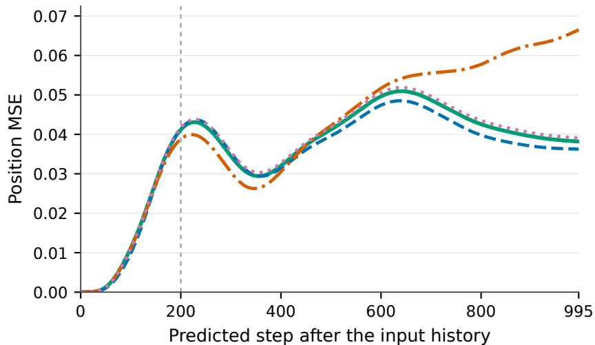
(a) WaterDrop: 995 predicted steps
