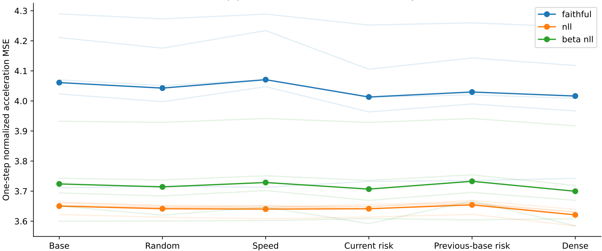
WaterDrop pilot: five seeds, three held-out trajectories
