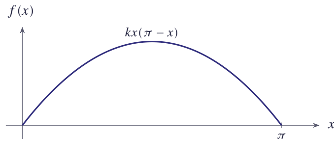
Figure 4.18 The parabolic initial profile f(x) = kx(\pi - x)
