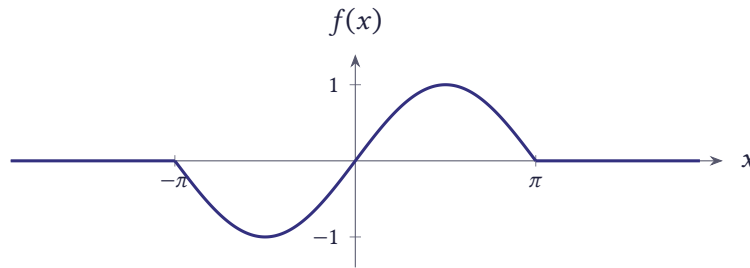
Figure 10.61 The function f(x) = \sin x for |x| \leq \pi and zero outside
