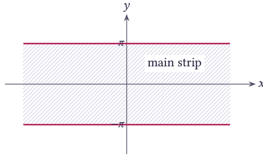
Figure 3.13 The fundamental strip of the hyperbolic functions: -\pi < y \leq \pi
