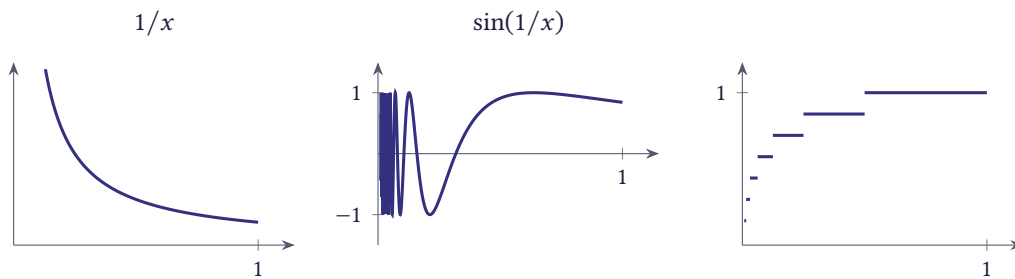
Figure 8.55 Functions that violate Dirichlet's conditions: 1/x (unbounded), \sin(1/x) (infinitely many maxima and minima) and a staircase function with infinitely many steps
