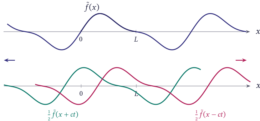
Figure 11.66 The odd periodic extension \tilde{f}(x) and the two waves \frac{1}{2}\tilde{f}(x + ct) and \frac{1}{2}\tilde{f}(x - ct) travelling in opposite directions
