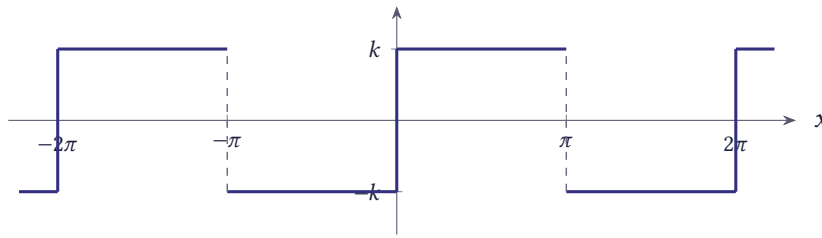
Figure 9.56 The square wave \pm k with period 2\pi used in the power example
