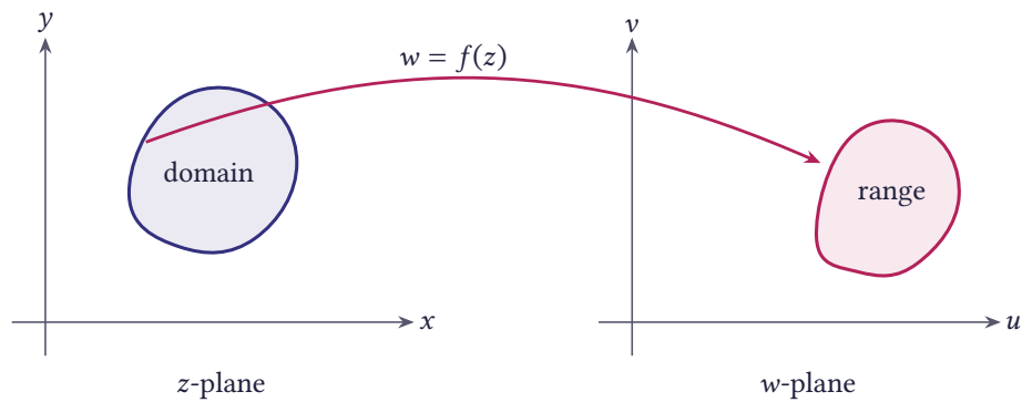
Figure 2.5 A complex function w = f(z) maps points of the domain in the z -plane to points of the range in the w -plane
