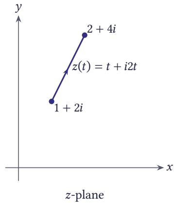
Figure 5.21 The path z(t) = t + i2t , 1 \leq t \leq 2
