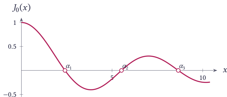
Figure 13.76 The function J_0(x) and its roots \alpha_1, \alpha_2, \alpha_3
