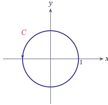
Figure 7.46 The unit circle z = e^{it} , 0 \leq t \leq 2\pi
