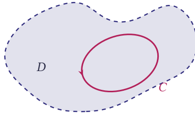
Figure 5.29 A simple closed path C in the simply connected domain D
