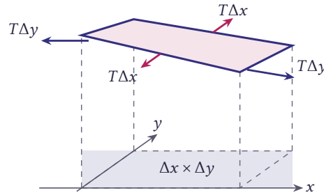
Figure 13.71 An element \Delta x \times \Delta y of the vibrating membrane and the tensile forces T\Delta x and T\Delta y acting on it
