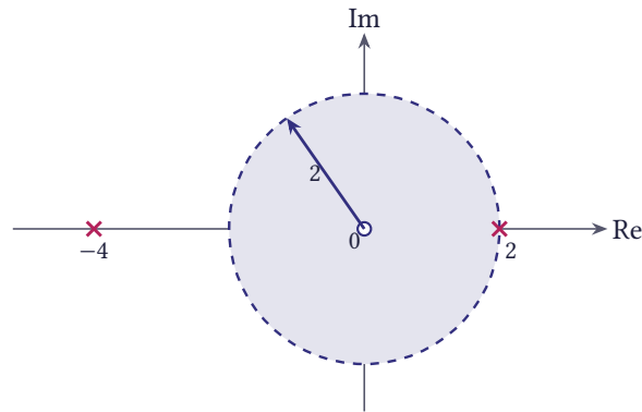
Figure 6.42 The poles z = -4 and z = 2 ; the circle of convergence about the origin has radius 2
