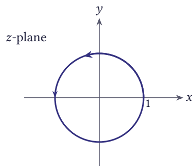
Figure 5.22 The path z(t) = e^{it} , 0 \leq t \leq 2\pi (the unit circle)
