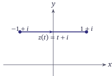
Figure 5.25 The path z(t) = t + i , -1 \leq t \leq 1 , from -1 + i to 1 + i
