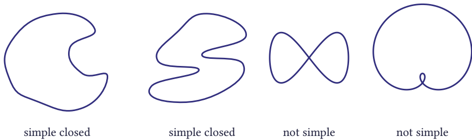
Figure 5.27 Simple closed curves and closed curves that are not simple
