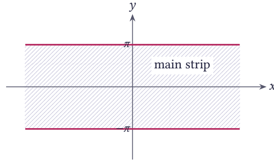
Figure 3.11 The fundamental strip of the exponential function: -\pi < y \leq \pi
