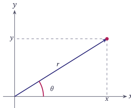
Figure 13.73 Polar coordinates: x = r \cos \theta , y = r \sin \theta
