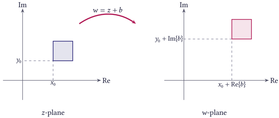
Figure 4.15 Translation w = z + b : a region of the z -plane is shifted by b without changing its shape
