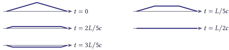
Figure 11.67 The solution of the example at t = 0, L/5c, 2L/5c, L/2c and 3L/5c ; at t = L/2c the string is flat
