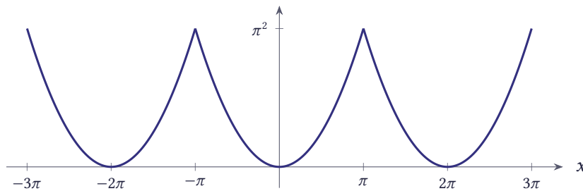
Figure 8.53 The function f(x) = x^2 on [-\pi, \pi] with its periodic extension
