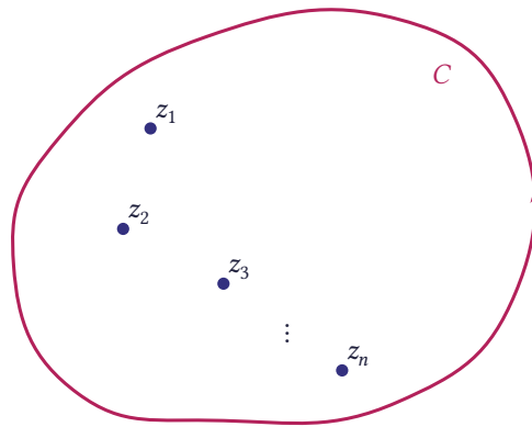
Figure 5.36 A path C and the non-analytic points z_1, \dots, z_n inside it
