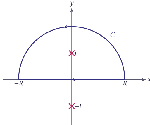
Figure 7.45 The upper semicircular path; the double pole z = i lies inside the path and z = -i outside it
