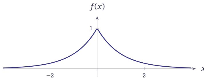
Figure 10.60 The function f(x) = e^{-|x|}
