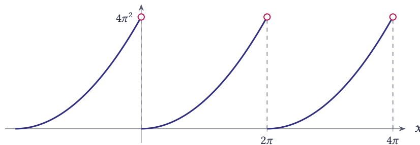
Figure 8.54 The function f(x) = x^2 on [0, 2\pi] with its periodic extension
