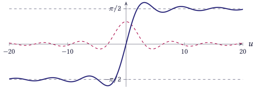
Figure 10.58 The function \text{Si}(u) (solid) and the function \sin u/u (dashed)
