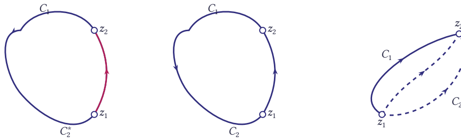
Figure 5.30 The paths C_1 , C_2 and C_2^* ( C_2 with reversed direction) between z_1 and z_2
