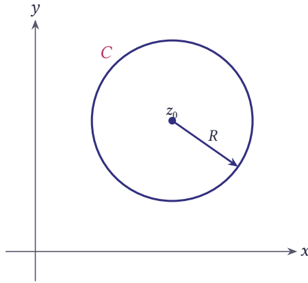
Figure 5.38 A circle C with centre z_0 and radius R
