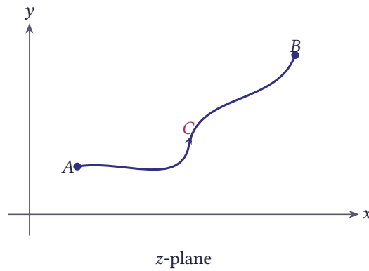
Figure 5.19 A path of integration C from the point A to the point B in the z -plane
