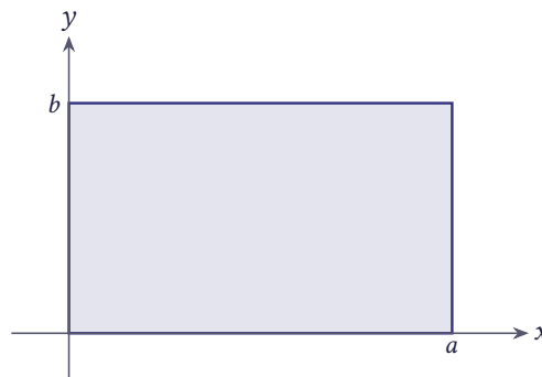
Figure 13.72 The rectangular region 0 \leq x \leq a, 0 \leq y \leq b
