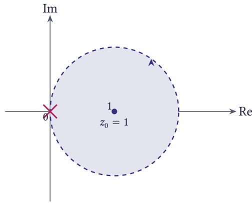
Figure 6.43 The region of convergence of the series about z_0 = 1 is a disc of radius 1 (up to the pole z = 0 )
