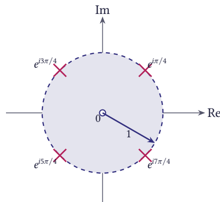
Figure 6.41 The four poles of z^4 + 1 = 0 on the unit circle; the radius of convergence of the series about the origin is 1
