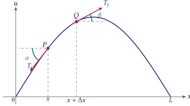
Figure 11.62 A segment PQ of the vibrating string: the tensions T_1 and T_2 at its ends, at angles \alpha and \beta
