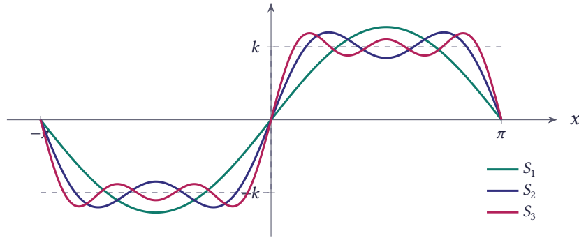
Figure 8.51 The partial sums S_1 , S_2 and S_3 of the Fourier series of the square wave (the dashed line is the square wave itself)
