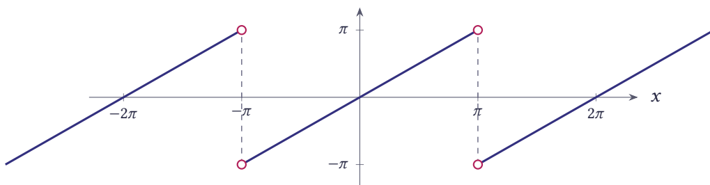
Figure 8.52 The sawtooth wave f(x) = x on [-\pi, \pi] with its periodic extension
