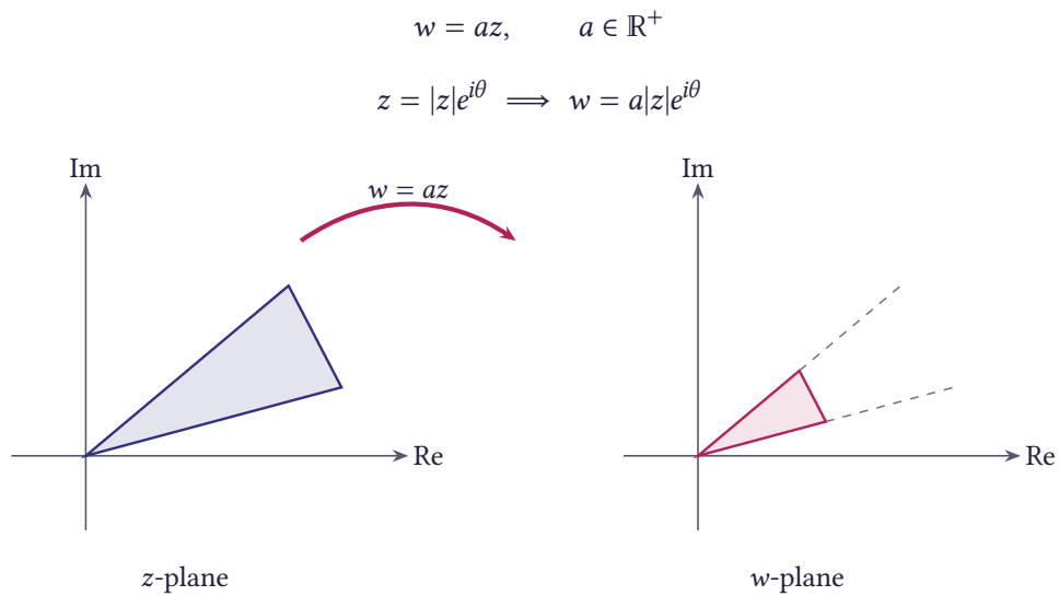
Figure 4.17 Contraction w = az with 0 < a < 1 ; for a > 1 the mapping is a dilation
