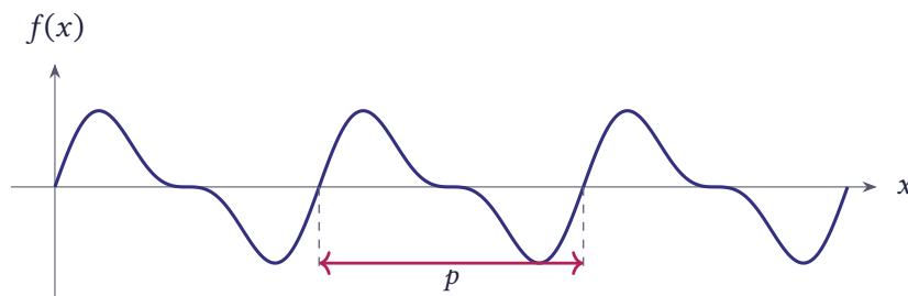
Figure 8.48 A periodic function with period p
