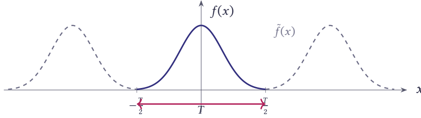
Figure 10.57 A non-periodic function f(x) and its periodic extension \tilde{f}(x) with period T
