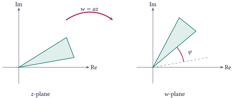
Figure 4.16 Rotation w = az with |a| = 1 : a region of the z -plane is rotated about the origin by \varphi = \arg a
