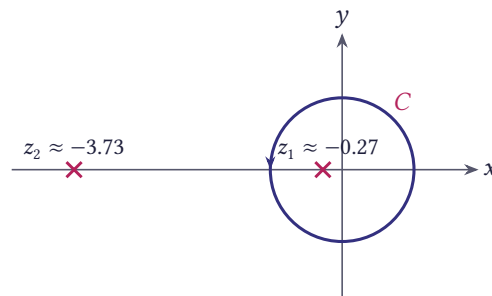
Figure 7.47 The unit circle and the poles z_1 \approx -0.27 (inside) and z_2 \approx -3.73 (outside)
