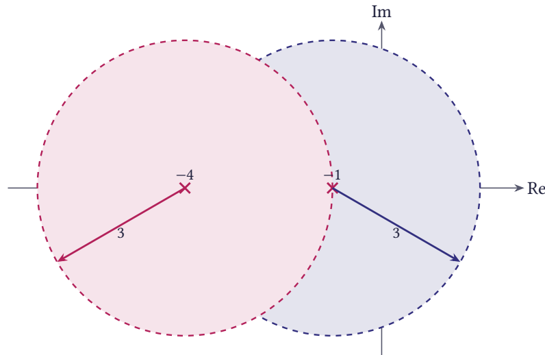
Figure 6.44 The poles z = -1 and z = -4 of f(z) = \frac{z}{(z+1)(z+4)^3}
