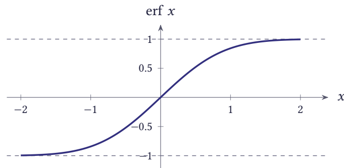
Figure 12.69 The graph of the error function \operatorname{erf}(x) for -2 \leq x \leq 2
