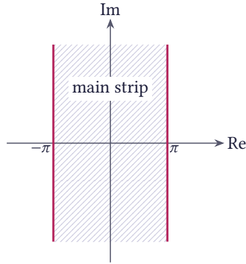
Figure 3.12 The fundamental strip of \sin z and \cos z : -\pi < x \leq \pi
