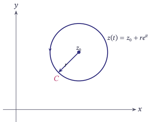
Figure 5.31 A circle C with centre z_0 and radius r
