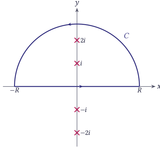
Figure 5.34 The semicircular path; the poles are at z = \pm i and z = \pm 2i
