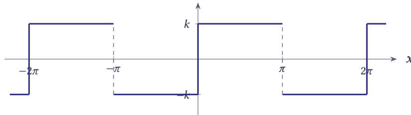
Figure 8.50 A square wave f(x) with period 2\pi and values \pm k
