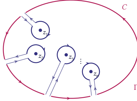
Figure 5.37 The path \Gamma for the proof: C , the circles C_1, \dots, C_n and the connecting segments
