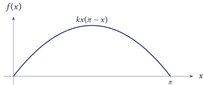
Figure 11.65 The parabolic initial profile f(x) = kx(\pi - x)
