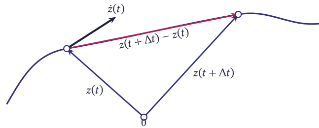
Figure 5.23 The derivative of the path \dot{z}(t) as the limit of \frac{z(t+\Delta t)-z(t)}{\Delta t}
