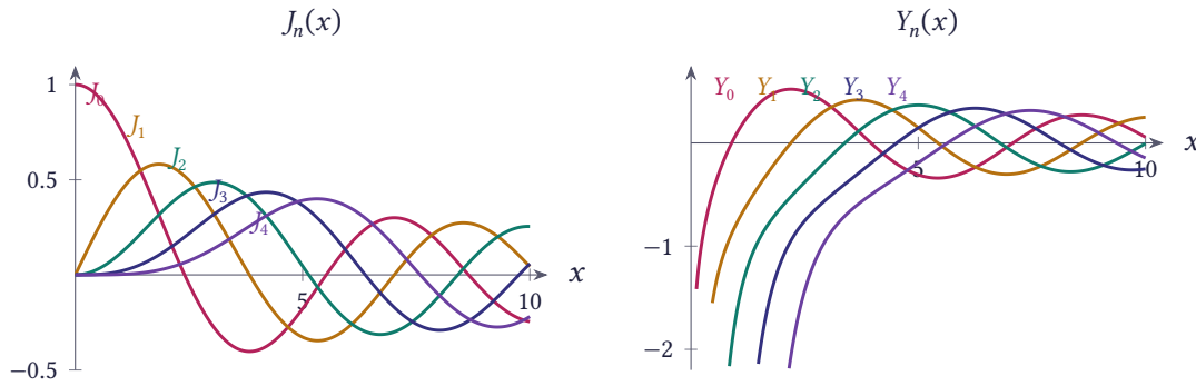
Figure 13.75 The Bessel functions of the first kind J_0, \dots, J_4 and of the second kind Y_0, \dots, Y_4 for 0 < x \leq 10
