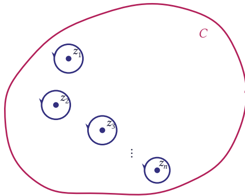
Figure 6.40 A path C and the singular points z_1, \dots, z_n inside it; a small circle is drawn around each point
