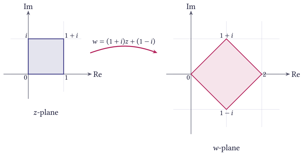
Figure 4.18 The image of the unit square under the mapping w = (1+i)z + (1-i)
