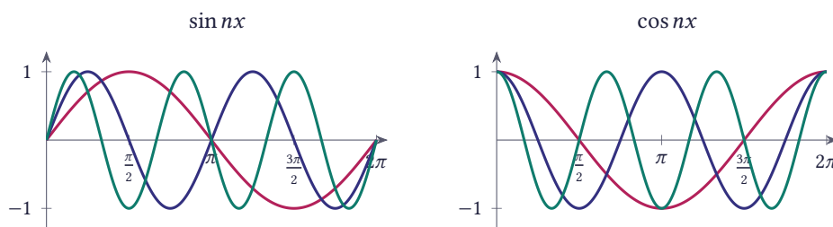
Figure 8.49 The functions \sin nx and \cos nx for n = 1, 2, 3 on [0, 2\pi]
