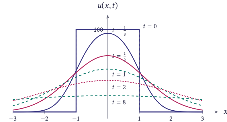
Figure 12.70 The temperature distribution u(x, t) at t = 0, \frac{1}{8}, \frac{1}{2}, 1, 2 and 8 for the initial pulse U_0 = 100 and c = 1
