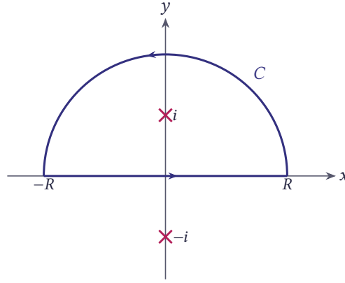
Figure 5.33 The semicircular path in the upper half-plane; the poles are at z = \pm i
