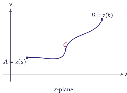
Figure 5.20 The path C , directed from A = z(a) to B = z(b)
