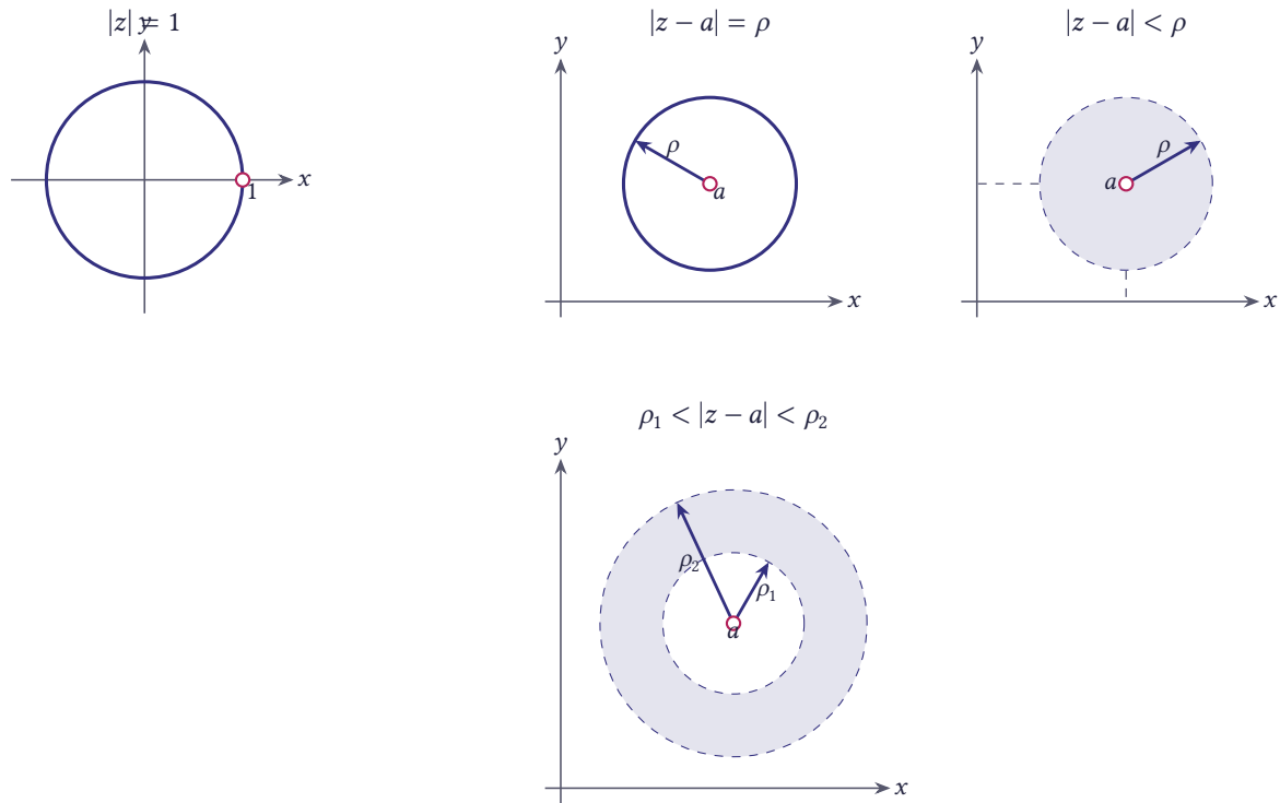
Figure 2.6 Important loci: a circle, the \rho -neighbourhood of a point a , and an annular region
