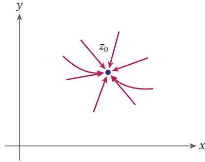
Figure 2.9 Approaching the point z_0 from all directions
