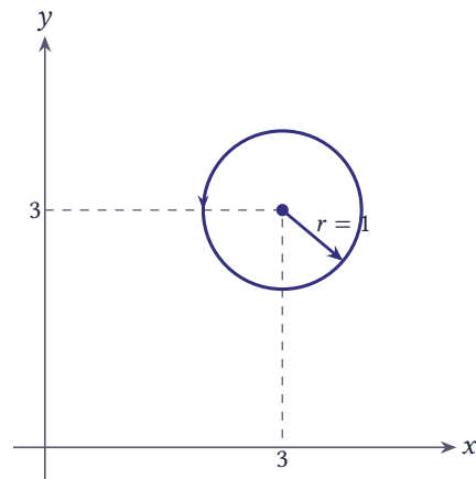
Figure 5.39 The path of exercise 4: a circle with centre 3 + 3i and radius r = 1
