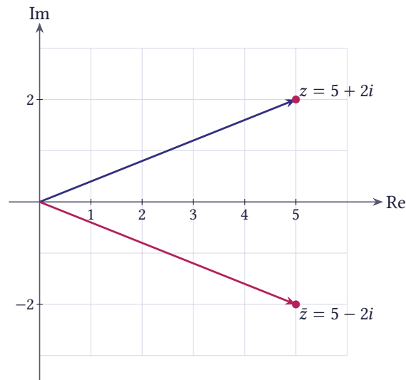
Figure 1.2 The complex number z = 5 + 2i and its conjugate \bar{z} = 5 - 2i
