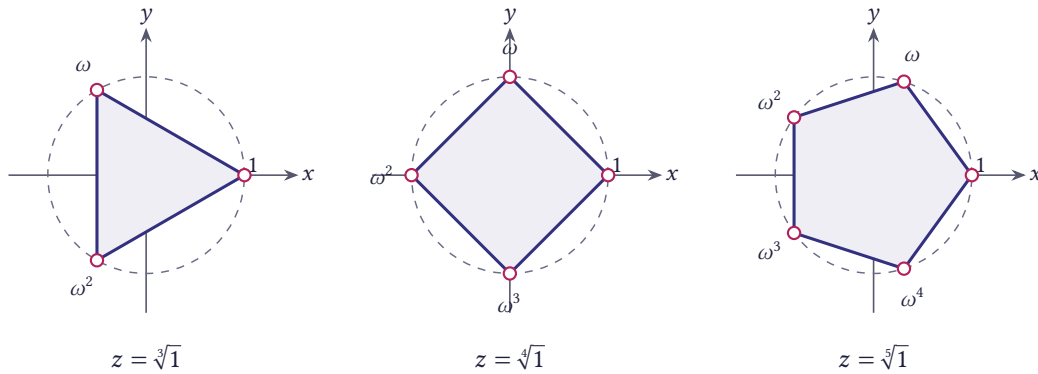
Figure 1.4 The roots z = \sqrt[3]{1} , z = \sqrt[4]{1} and z = \sqrt[5]{1} on the unit circle
