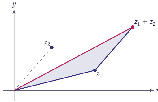
Figure 1.3 The triangle inequality: a triangle with vertices 0, z_1 and z_1 + z_2
