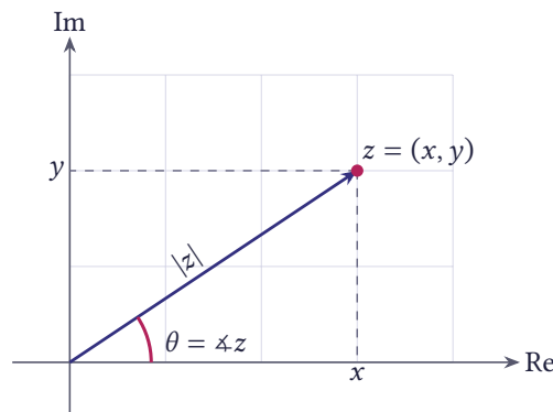
Figure 1.1 The complex number z = (x, y) in the complex plane; its modulus |z| and argument \theta
