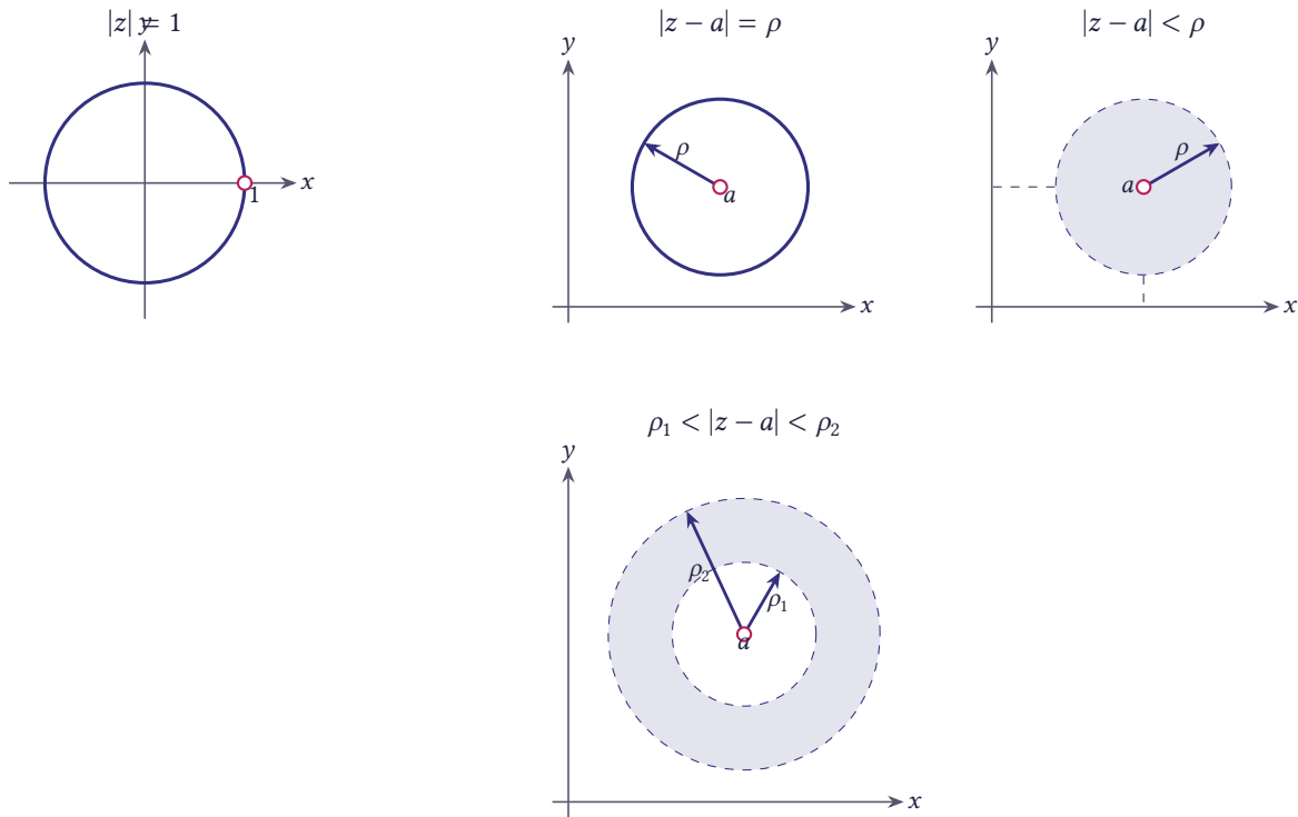
Figure 2.2 Important loci: a circle, the \rho -neighbourhood of a point a , and an annular region
