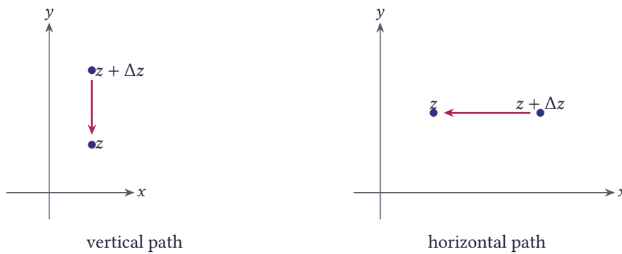
Figure 2.6 Two paths towards z : the vertical direction ( \Delta z = i\Delta y ) and the horizontal direction ( \Delta z = \Delta x )
