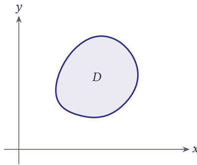
Figure 2.4 A domain D in the complex plane
