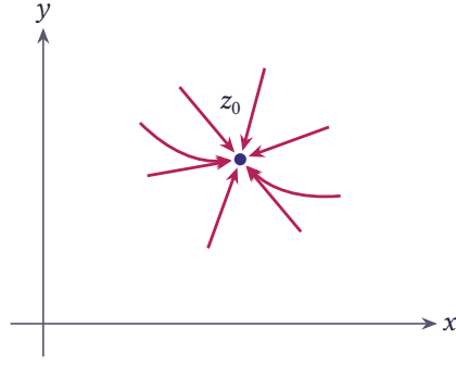
Figure 2.5 Approaching the point z_0 from all directions
