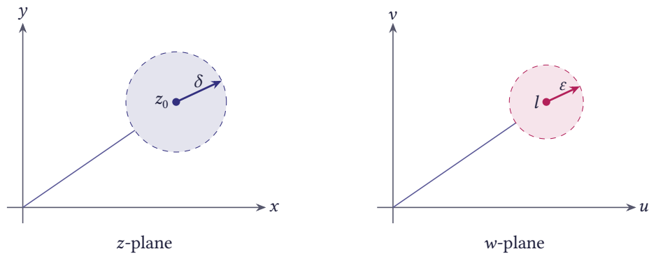
Figure 2.3 The definition of the limit: the \delta -neighbourhood of z_0 in the z -plane and the \varepsilon -neighbourhood of l in the w -plane
