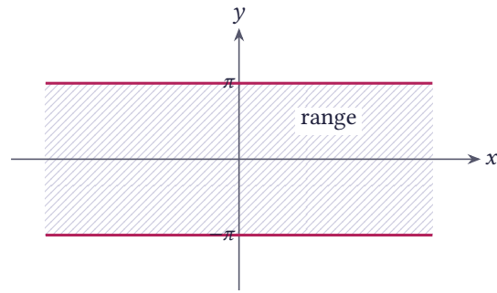
Figure 3.4 The range of the logarithm function: the strip -\pi < \text{Im } w \leq \pi
