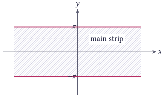
Figure 3.1 The fundamental strip of the exponential function: -\pi < y \leq \pi
