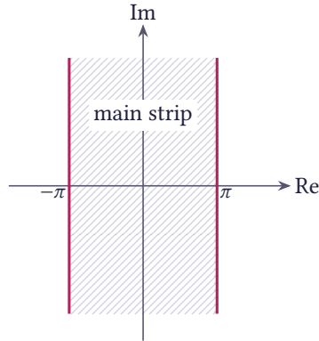
Figure 3.2 The fundamental strip of \sin z and \cos z : -\pi < x \leq \pi
