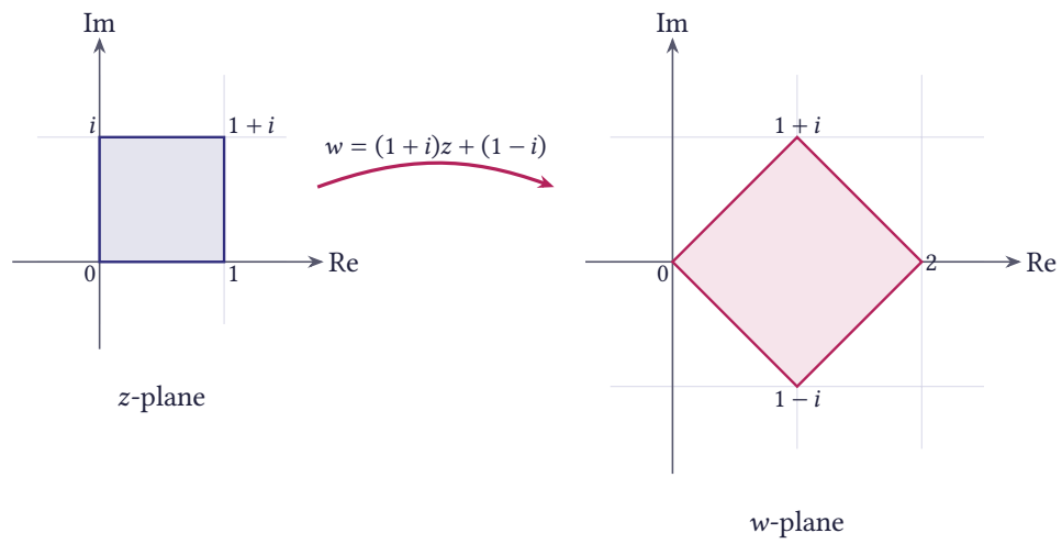
Figure 4.4 The image of the unit square under the mapping w = (1+i)z + (1-i)
