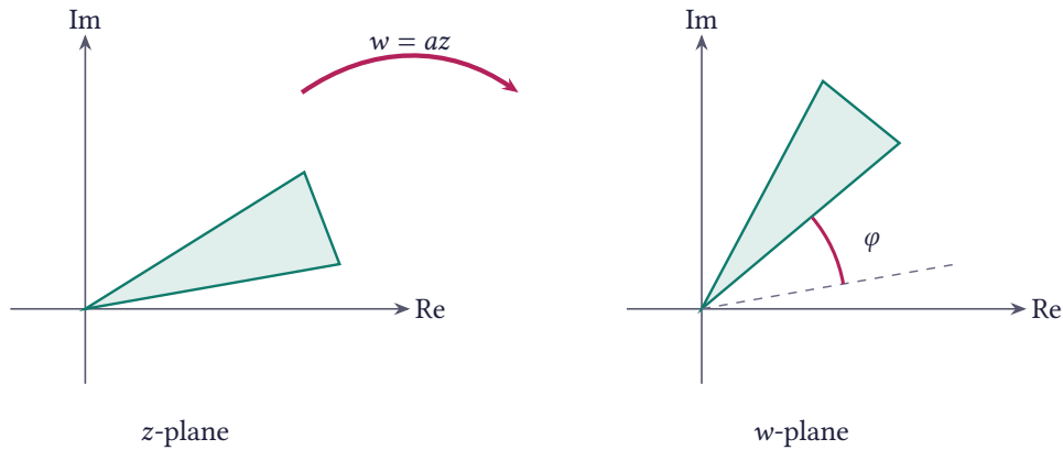
Figure 4.2 Rotation w = az with |a| = 1 : a region of the z -plane is rotated about the origin by \varphi = \arg a
