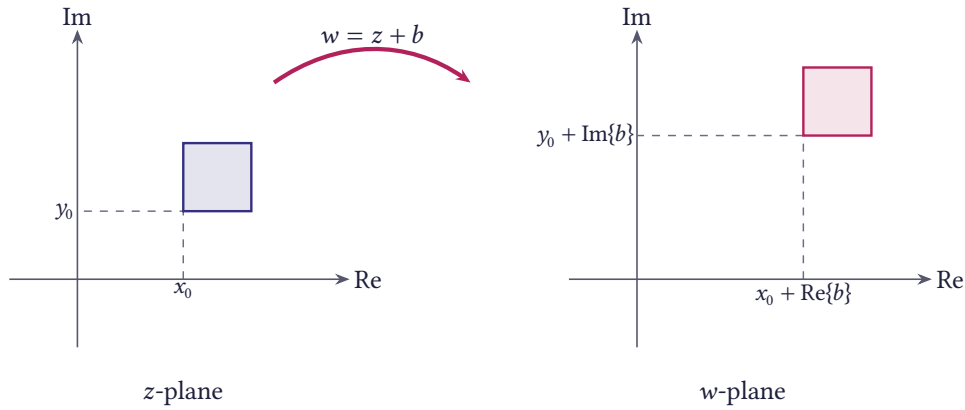
Figure 4.1 Translation w = z + b : a region of the z -plane is shifted by b without changing its shape
