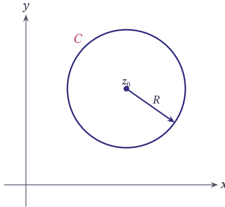
Figure 5.20 A circle C with centre z_0 and radius R
