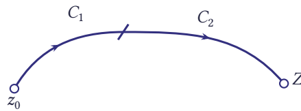
Figure 5.8 A path C from z_0 to Z split into two pieces C_1 and C_2
