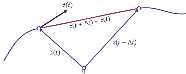
Figure 5.5 The derivative of the path \dot{z}(t) as the limit of \frac{z(t+\Delta t) - z(t)}{\Delta t}
