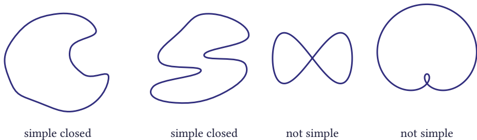
Figure 5.9 Simple closed curves and closed curves that are not simple
