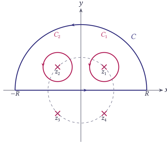
Figure 5.17 The semicircular path and the circles C_1 and C_2 around the poles z_1 and z_2 ; the poles z_3 and z_4 lie in the lower half-plane
