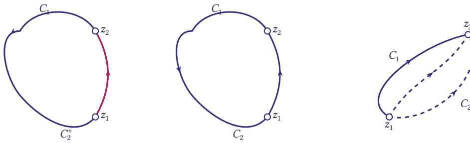
Figure 5.12 The paths C_1 , C_2 and C_2^* ( C_2 with reversed direction) between z_1 and z_2
