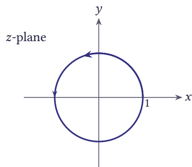
Figure 5.4 The path z(t) = e^{it} , 0 \leq t \leq 2\pi (the unit circle)
