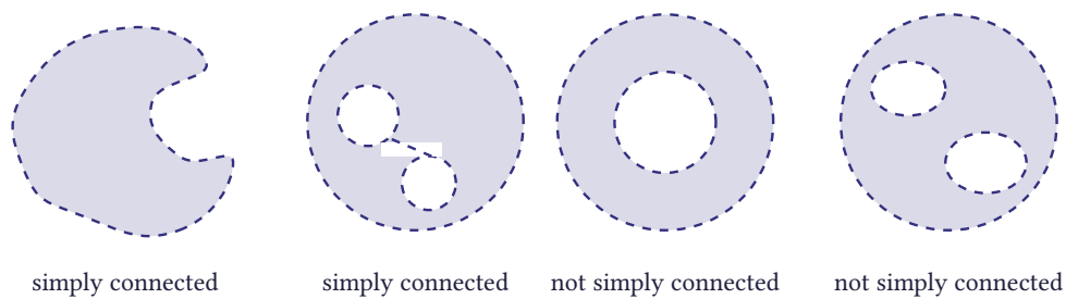
Figure 5.10 Simply connected and not simply connected domains
