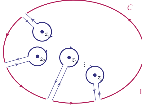
Figure 5.19 The path \Gamma for the proof: C , the circles C_1, \dots, C_n and the connecting segments
