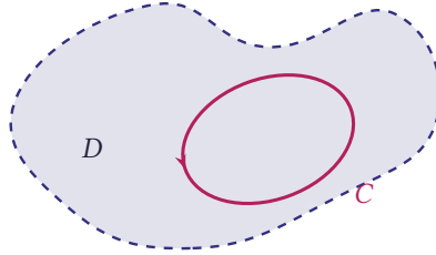
Figure 5.11 A simple closed path C in the simply connected domain D
