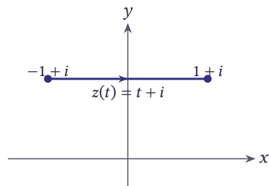
Figure 5.7 The path z(t) = t + i , -1 \leq t \leq 1 , from -1 + i to 1 + i
