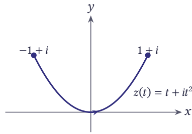
Figure 5.6 The path z(t) = t + it^2 , -1 \leq t \leq 1 , from -1 + i to 1 + i
