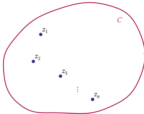
Figure 5.18 A path C and the non-analytic points z_1, \dots, z_n inside it
