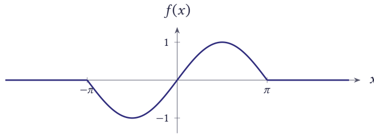
Figure 10.5 The function f(x) = \sin x for |x| \leq \pi and zero outside
