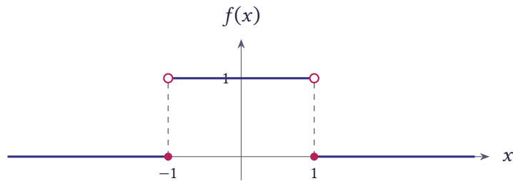
Figure 10.3 The rectangular pulse f(x) = 1 for |x| < 1
