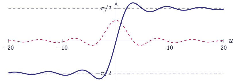
Figure 10.2 The function \text{Si}(u) (solid) and the function \sin u/u (dashed)
