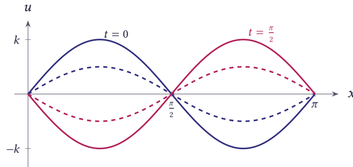
Figure 11.2 The second mode of the string: u(x, t) = k \sin 2x \cos 2t at different times
