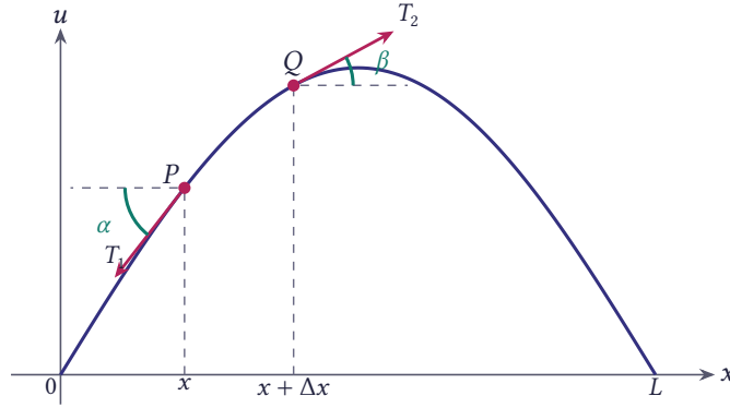
Figure 11.1 A segment PQ of the vibrating string: the tensions T_1 and T_2 at its ends, at angles \alpha and \beta
