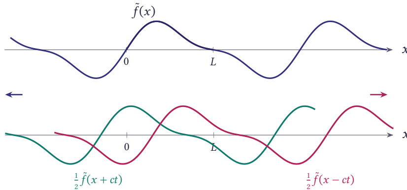
Figure 11.5 The odd periodic extension \tilde{f}(x) and the two waves \frac{1}{2}\tilde{f}(x + ct) and \frac{1}{2}\tilde{f}(x - ct) travelling in opposite directions
