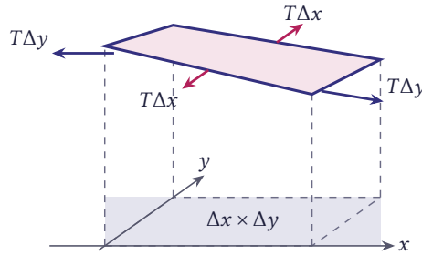
Figure 13.1 An element \Delta x \times \Delta y of the vibrating membrane and the tensile forces T\Delta x and T\Delta y acting on it
