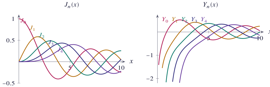
Figure 6.5 The Bessel functions of the first kind J_0, \dots, J_4 and of the second kind Y_0, \dots, Y_4 for 0 < x \leq 10
