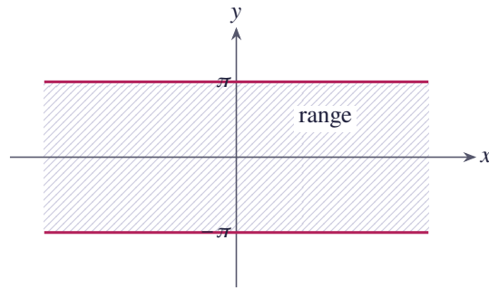
Figure 10.4 The range of the logarithm function: the strip -\pi < \operatorname{Im} w \leq \pi
