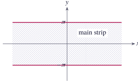
Figure 10.1 The fundamental strip of the exponential function: -\pi < y \leq \pi
