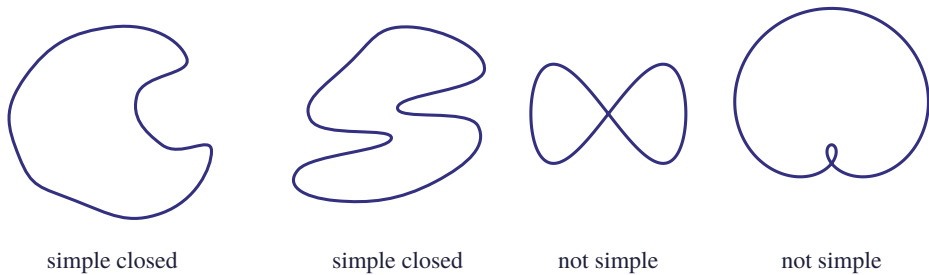
Figure 12.9 Simple closed curves and closed curves that are not simple
