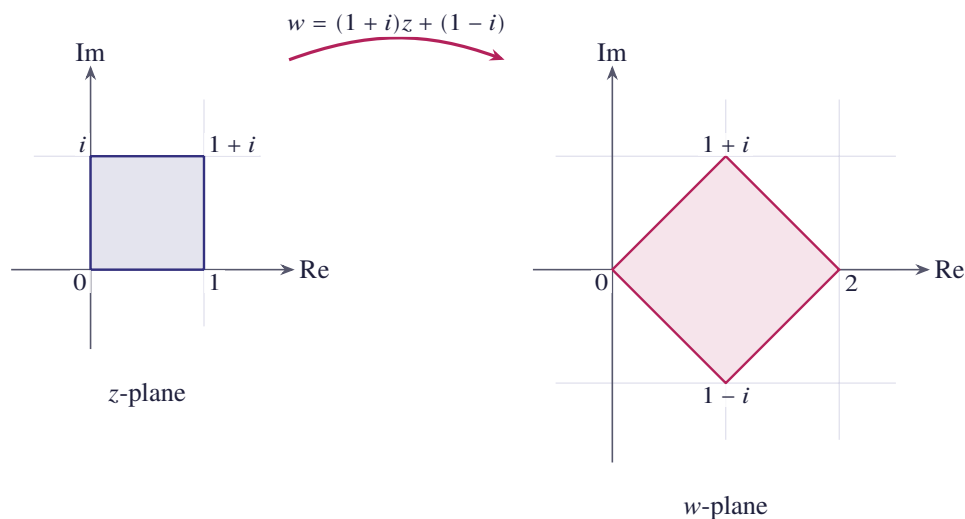
Figure 11.48 The image of the unit square under the mapping w = (1 + i)z + (1 - i)
