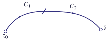
Figure 12.56 A path C from z_0 to Z split into two pieces C_1 and C_2
