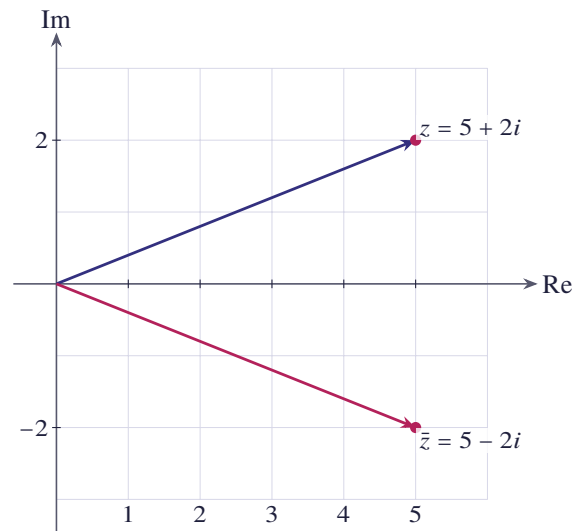
Figure 8.32 The complex number z = 5 + 2i and its conjugate \bar{z} = 5 - 2i
