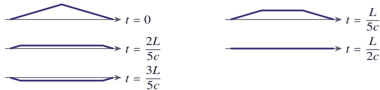
Figure 4.20 The solution of the example at t = 0 , \frac{L}{5c} , \frac{2L}{5c} , \frac{L}{2c} and \frac{3L}{5c} ; at t = \frac{L}{2c} the string is flat
