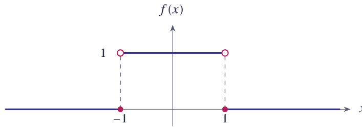
Figure 3.12 The rectangular pulse f(x) = 1 for |x| < 1
