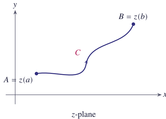
Figure 12.50 The path C , directed from A = z(a) to B = z(b)
