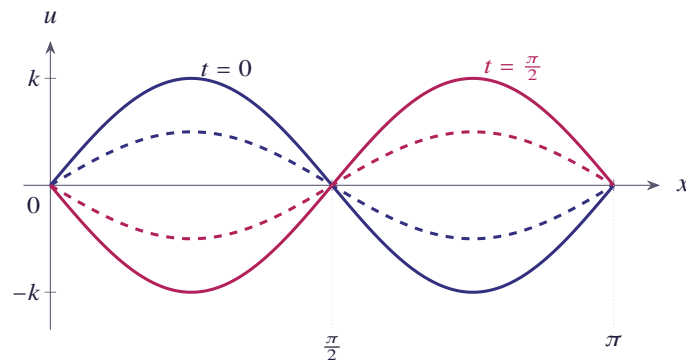
Figure 4.16 The second mode of the string: u(x, t) = k \sin 2x \cos 2t at different times
