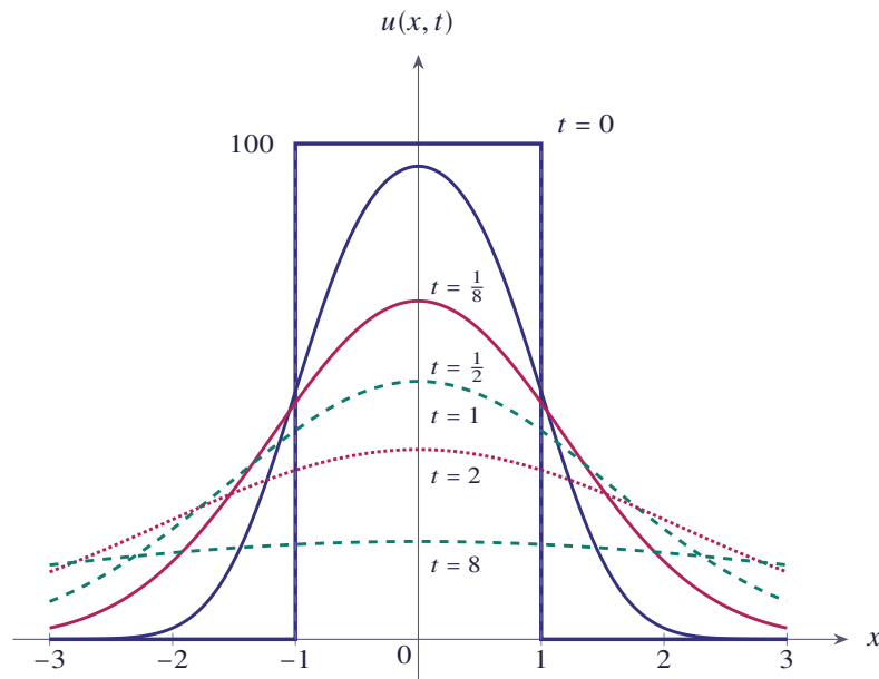
Figure 5.23 The temperature distribution u(x, t) at t = 0, \frac{1}{8}, \frac{1}{2}, 1, 2 and 8 for the initial pulse U_0 = 100 and c = 1
