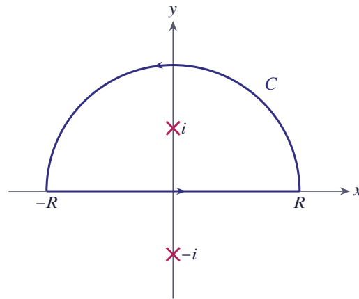
Figure 14.75 The upper semicircular path; the double pole z = i lies inside the path and z = -i outside it
