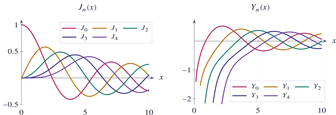
Figure 6.28 The Bessel functions of the first kind J_0, \dots, J_4 and of the second kind Y_0, \dots, Y_4 for 0 < x \leq 10
