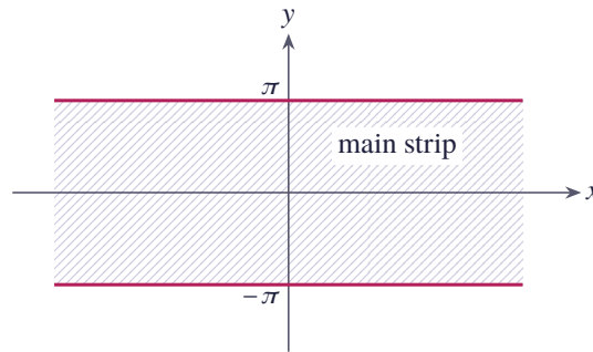
Figure 10.43 The fundamental strip of the hyperbolic functions: -\pi < y \leq \pi
