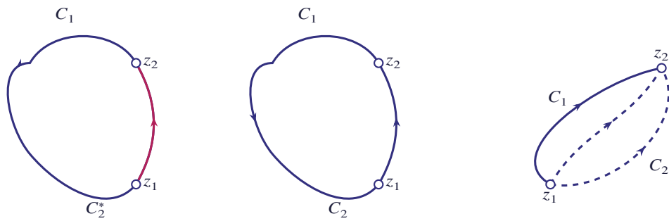
Figure 12.60 The paths C_1 , C_2 and C_2^* ( C_2 with reversed direction) between z_1 and z_2
