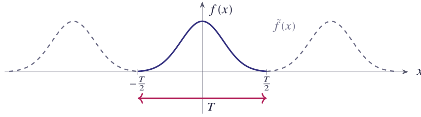
Figure 3.10 A non-periodic function f(x) and its periodic extension \tilde{f}(x) with period T
