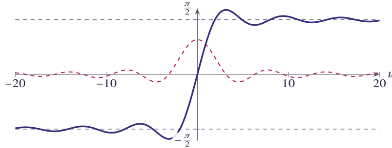
Figure 3.11 The function \text{Si}(u) (solid) and the function \frac{\sin u}{u} (dashed)
