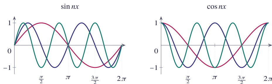
Figure 1.2 The functions \sin nx and \cos nx for n = 1, 2, 3 on [0, 2\pi]
