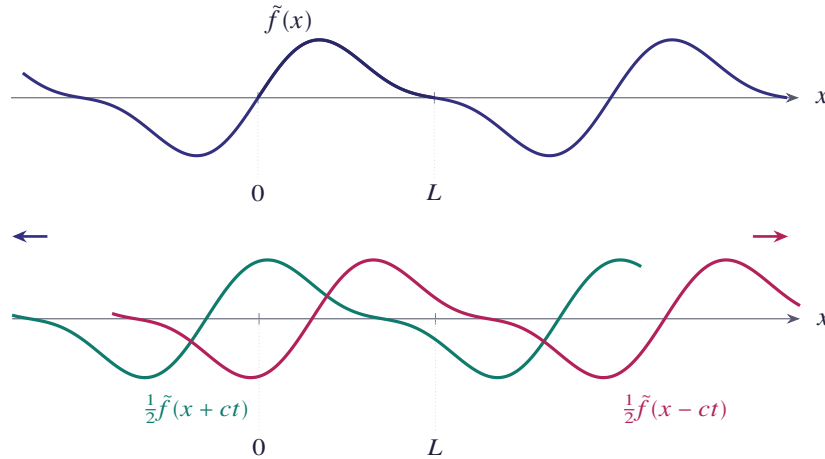
Figure 4.19 The odd periodic extension \tilde{f}(x) and the two waves \frac{1}{2}\tilde{f}(x + ct) and \frac{1}{2}\tilde{f}(x - ct) travelling in opposite directions
