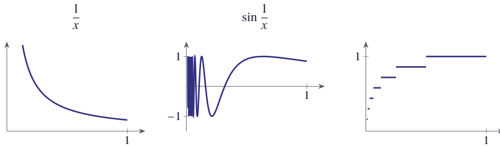
Figure 1.8 Functions that violate Dirichlet's conditions: \frac{1}{x} (unbounded), \sin \frac{1}{x} (infinitely many maxima and minima) and a staircase function with infinitely many steps
