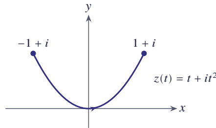
Figure 12.54 The path z(t) = t + it^2 , -1 \leq t \leq 1 , from -1 + i to 1 + i
