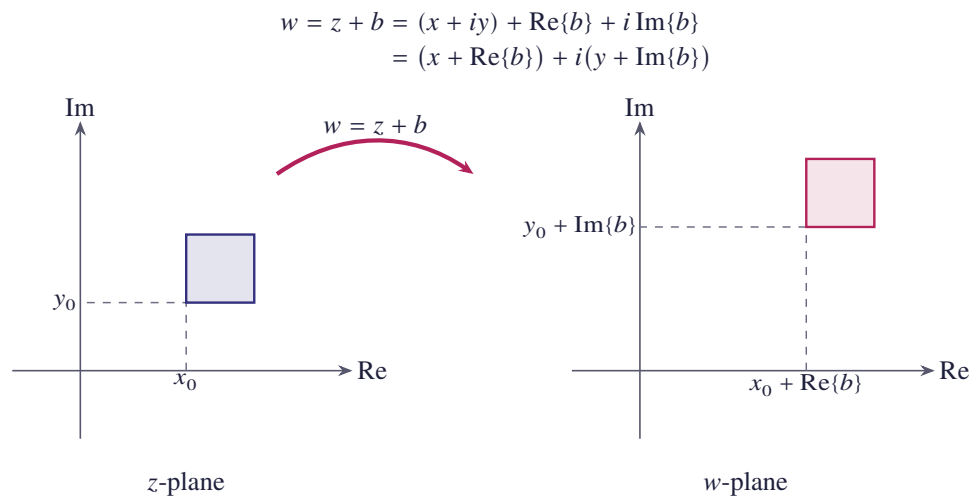
Figure 11.45 Translation w = z + b : a region of the z -plane is shifted by b without changing its shape
