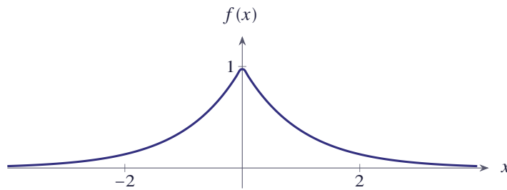
Figure 3.13 The function f(x) = e^{-|x|}
