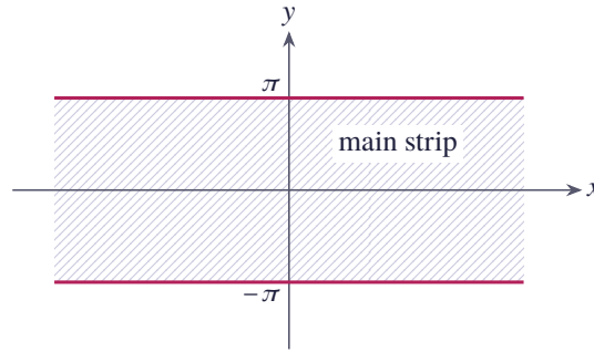
Figure 10.41 The fundamental strip of the exponential function: -\pi < y \leq \pi
