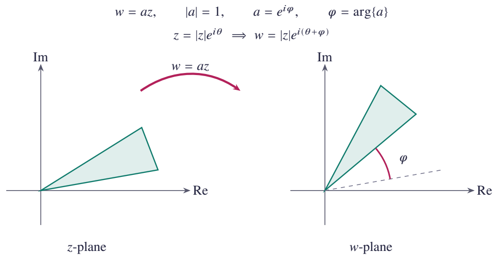
Figure 11.46 Rotation w = az with |a| = 1 : a region of the z -plane is rotated about the origin by \varphi = \arg a
