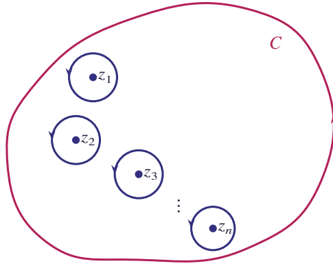
Figure 13.70 A path C and the singular points z_1, \dots, z_n inside it; a small circle is drawn around each point
