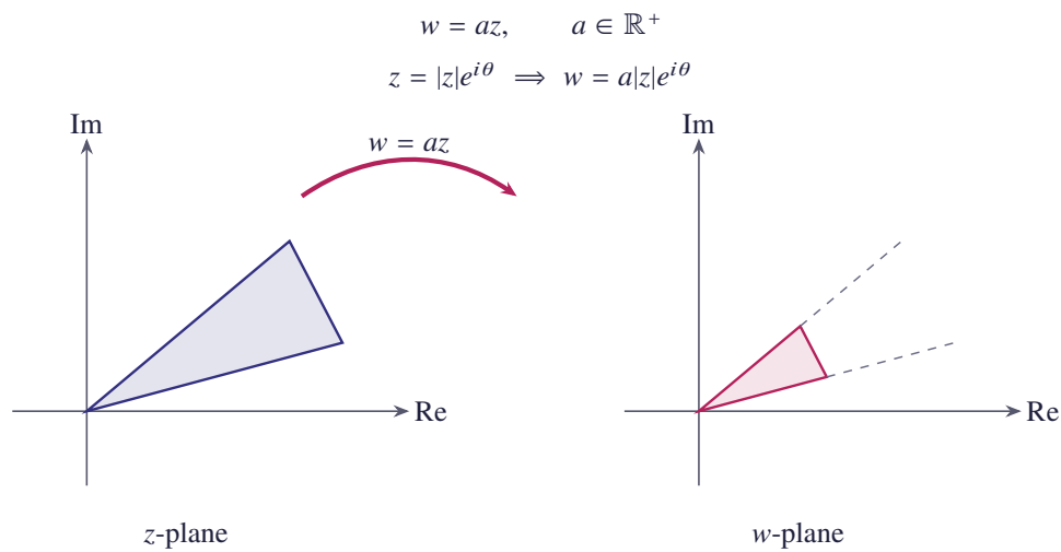
Figure 11.47 Contraction w = az with 0 < a < 1 ; for a > 1 the mapping is a dilation
