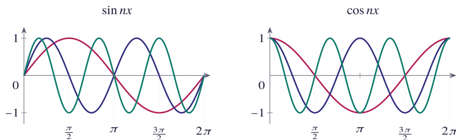
Figure 1.2 The functions \sin nx and \cos nx for n = 1, 2, 3 on [0, 2\pi]
